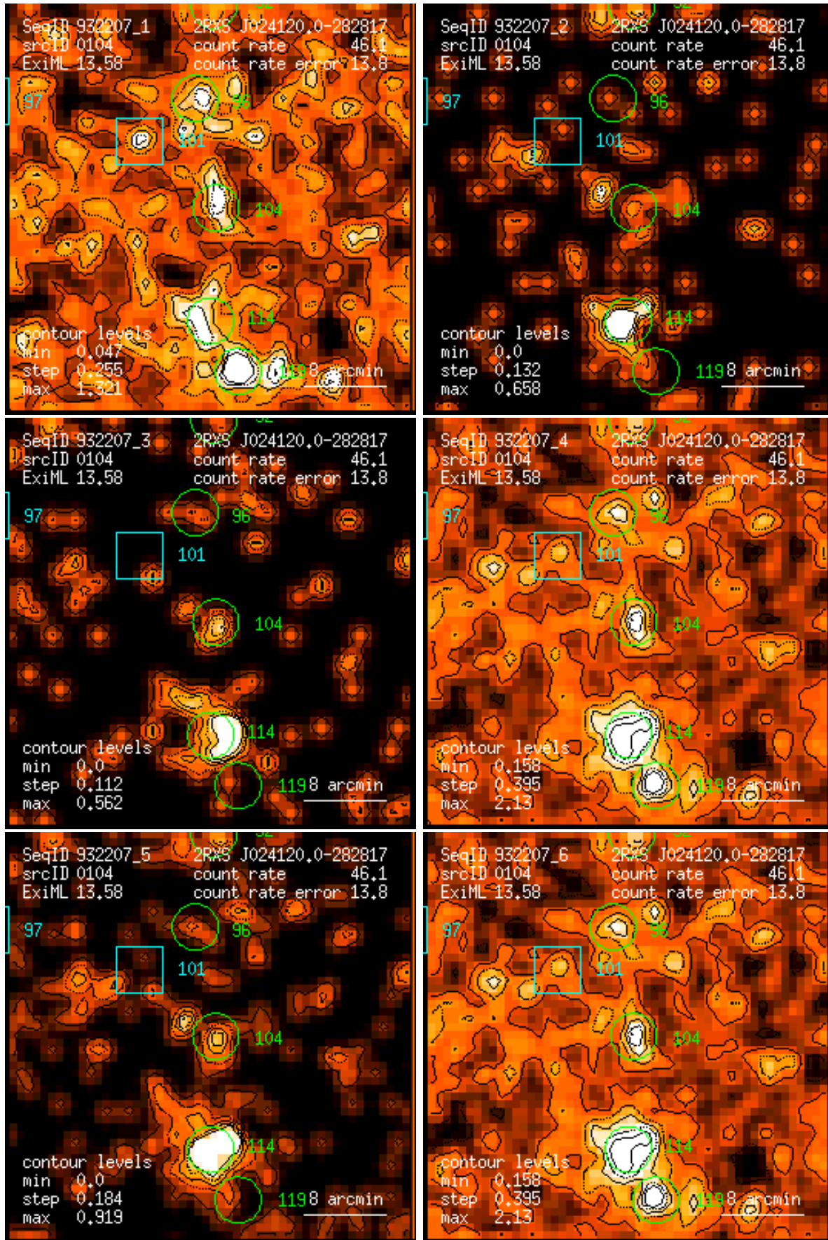
Figure 104: RASS 932207: detection 0104: band rate images, Gaussian filter: (1) PSPC channels 11 – 41, (2) 52 – 90, (3) 91 – 201, (4) 11 – 235, (5) 52 – 201, (6) 11 – 201. Broad band rates in counts/ks. Band rate contour levels in counts/ks/arcmin 2 .
