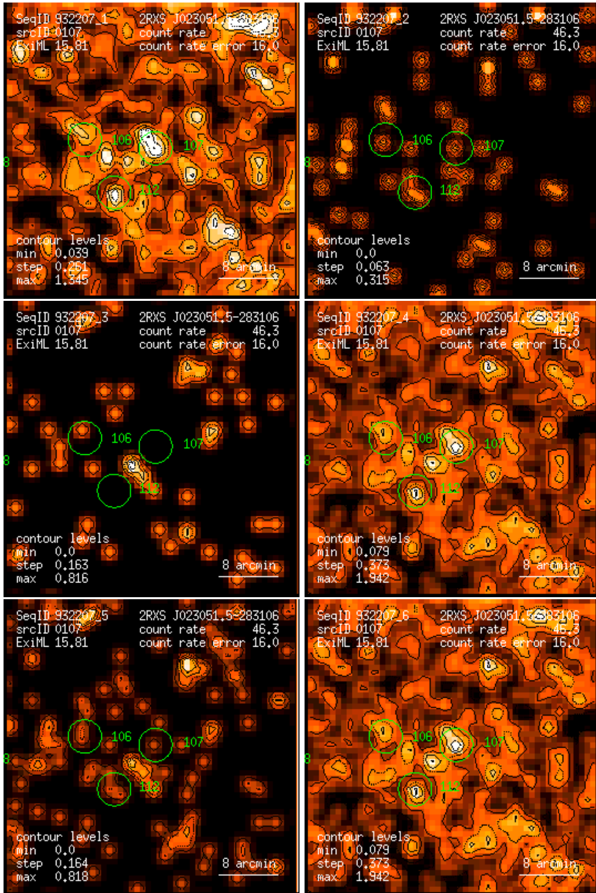
Figure 107: RASS 932207: detection 0107: band rate images, Gaussian filter: (1) PSPC channels 11 – 41, (2) 52 – 90, (3) 91 – 201, (4) 11 – 235, (5) 52 – 201, (6) 11 – 201. Broad band rates in counts/ks. Band rate contour levels in counts/ks/arcmin 2 .
