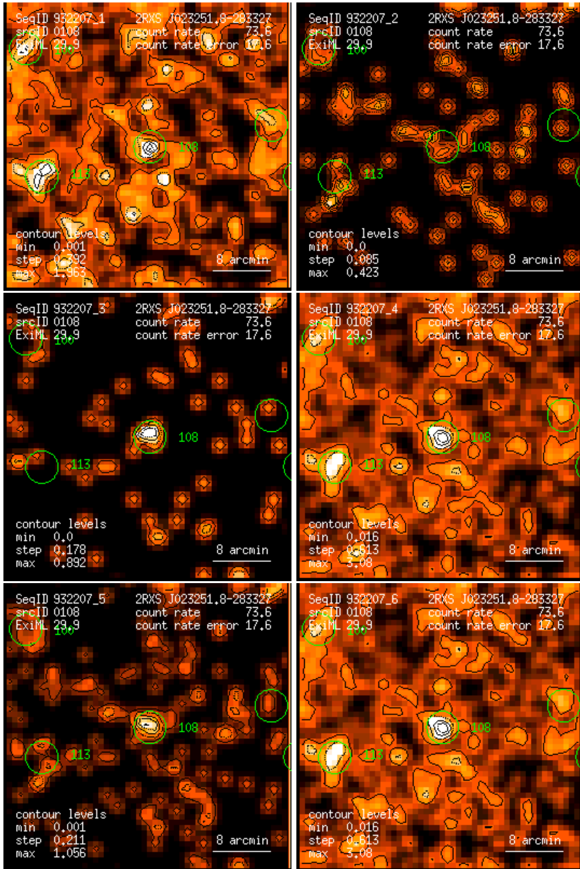
Figure 108: RASS 932207: detection 0108: band rate images, Gaussian filter: (1) PSPC channels 11 – 41, (2) 52 – 90, (3) 91 – 201, (4) 11 – 235, (5) 52 – 201, (6) 11 – 201. Broad band rates in counts/ks. Band rate contour levels in counts/ks/arcmin 2 .
