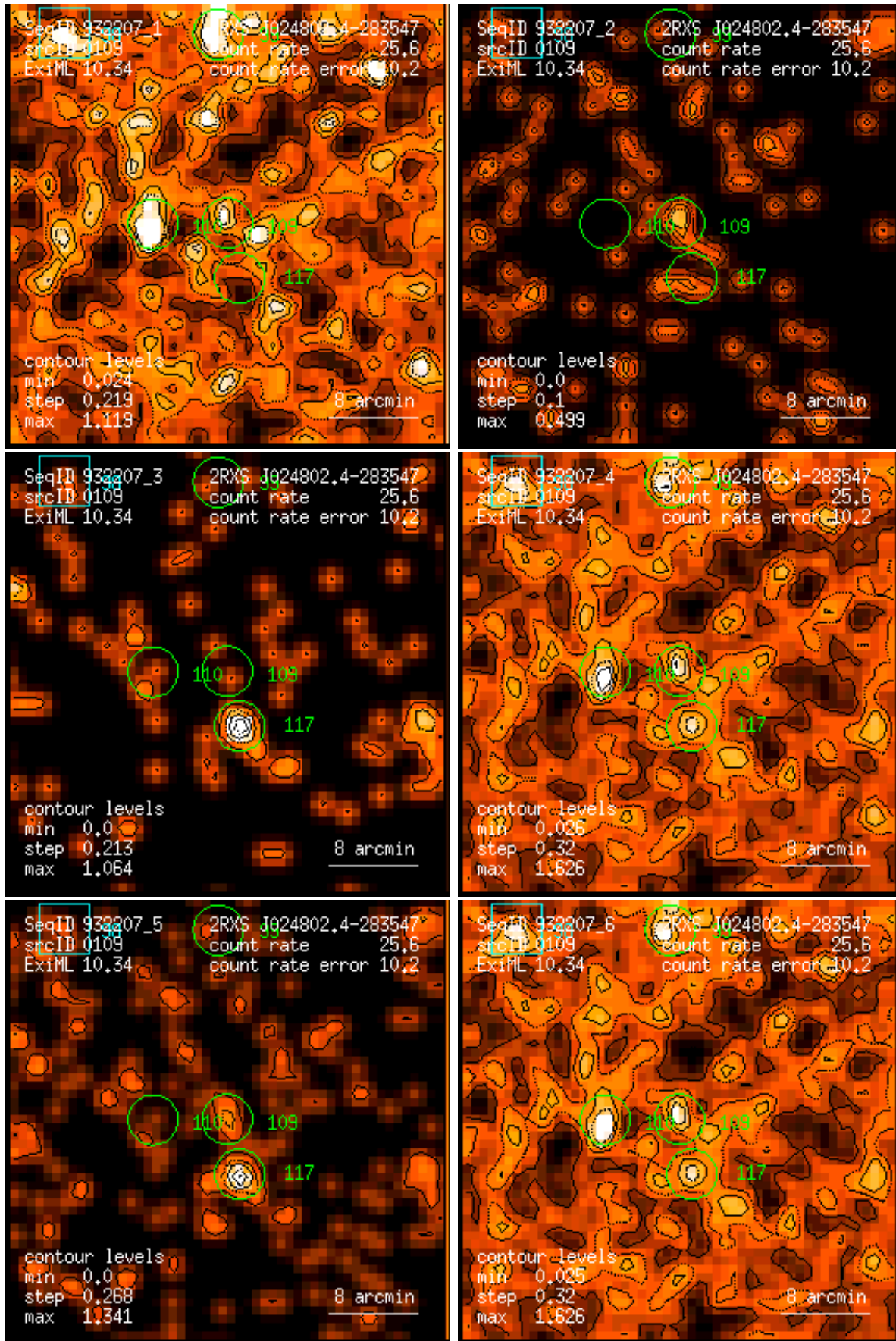
Figure 109: RASS 932207: detection 0109: band rate images, Gaussian filter: (1) PSPC channels 11 – 41, (2) 52 – 90, (3) 91 – 201, (4) 11 – 235, (5) 52 – 201, (6) 11 – 201. Broad band rates in counts/ks. Band rate contour levels in counts/ks/arcmin 2 .
