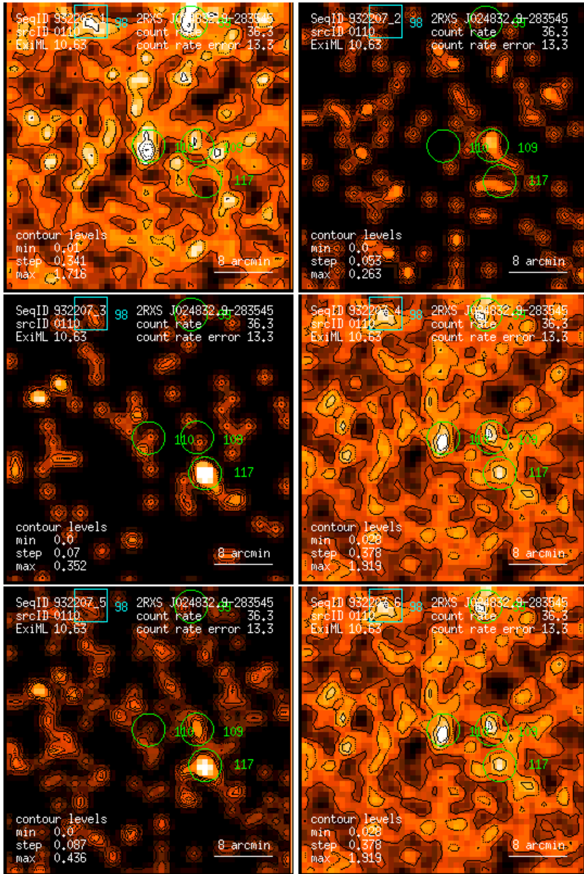
Figure 110: RASS 932207: detection 0110: band rate images, Gaussian filter: (1) PSPC channels 11 – 41, (2) 52 – 90, (3) 91 – 201, (4) 11 – 235, (5) 52 – 201, (6) 11 – 201. Broad band rates in counts/ks. Band rate contour levels in counts/ks/arcmin 2 .
