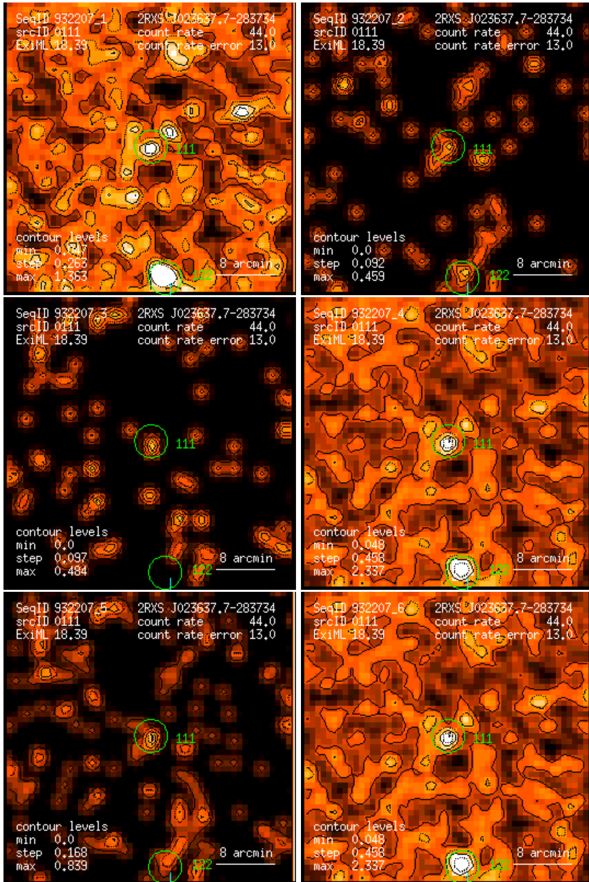
Figure 111: RASS 932207: detection 0111: band rate images, Gaussian filter: (1) PSPC channels 11 – 41, (2) 52 – 90, (3) 91 – 201, (4) 11 – 235, (5) 52 – 201, (6) 11 – 201. Broad band rates in counts/ks. Band rate contour levels in counts/ks/arcmin 2 .
