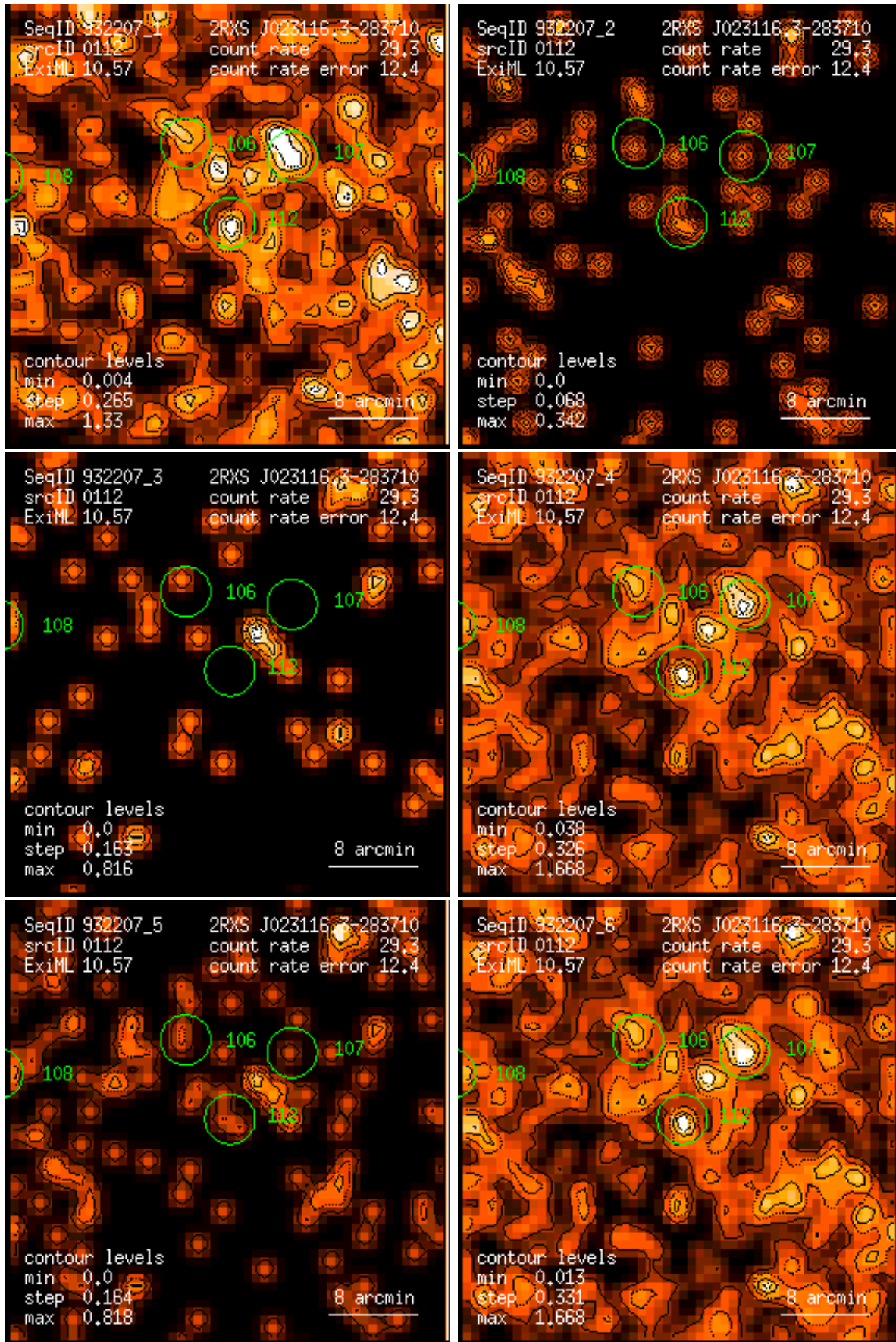
Figure 112: RASS 932207: detection 0112: band rate images, Gaussian filter: (1) PSPC channels 11 – 41, (2) 52 – 90, (3) 91 – 201, (4) 11 – 235, (5) 52 – 201, (6) 11 – 201. Broad band rates in counts/ks. Band rate contour levels in counts/ks/arcmin 2 .
