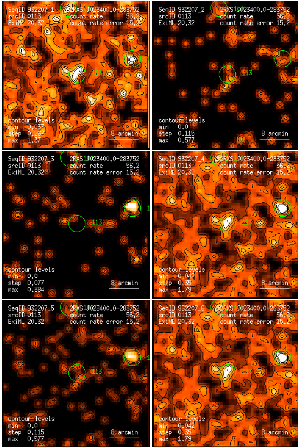
Figure 113: RASS 932207: detection 0113: band rate images, Gaussian filter: (1) PSPC channels 11 – 41, (2) 52 – 90, (3) 91 – 201, (4) 11 – 235, (5) 52 – 201, (6) 11 – 201. Broad band rates in counts/ks. Band rate contour levels in counts/ks/arcmin 2 .
