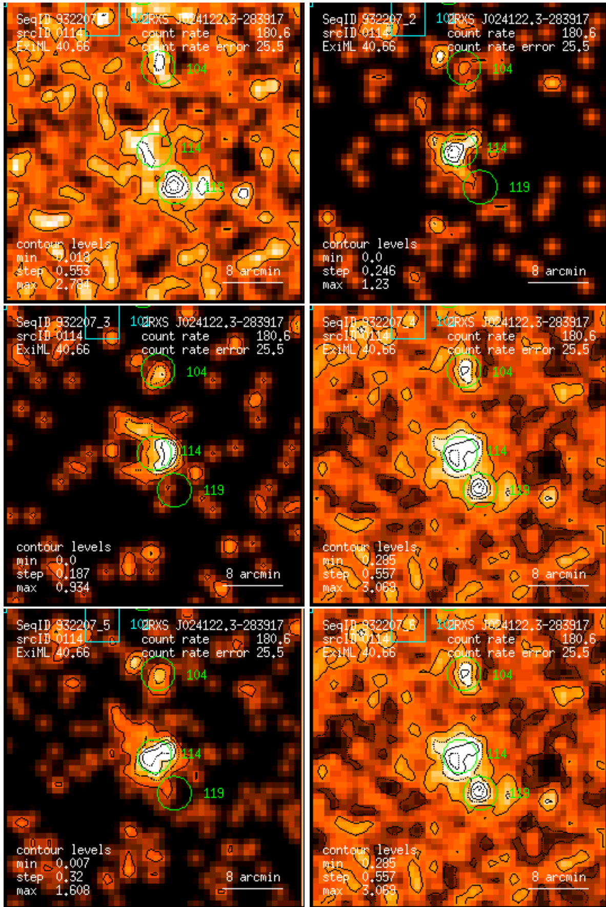
Figure 114: RASS 932207: detection 0114: band rate images, Gaussian filter: (1) PSPC channels 11 – 41, (2) 52 – 90, (3) 91 – 201, (4) 11 – 235, (5) 52 – 201, (6) 11 – 201. Broad band rates in counts/ks. Band rate contour levels in counts/ks/arcmin 2 .
