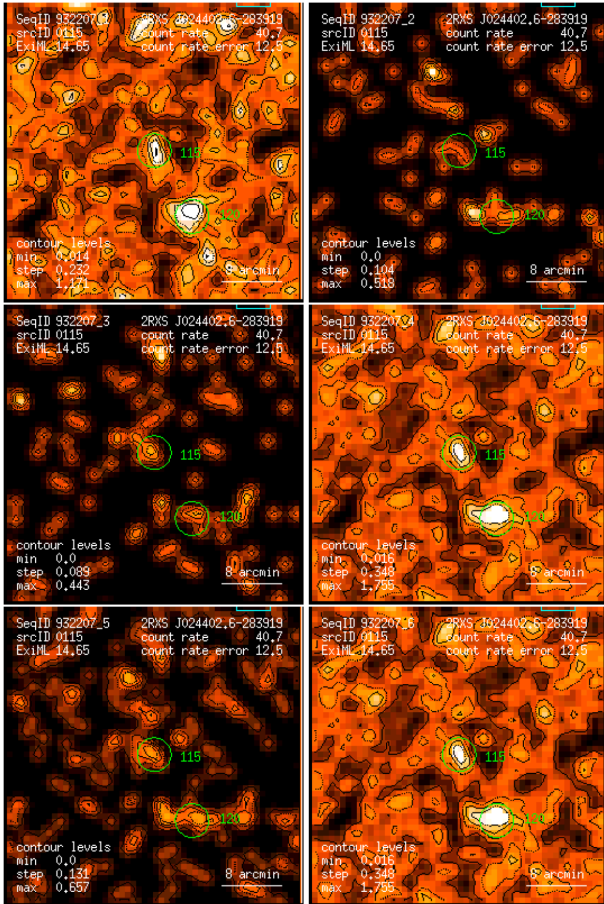
Figure 115: RASS 932207: detection 0115: band rate images, Gaussian filter: (1) PSPC channels 11 – 41, (2) 52 – 90, (3) 91 – 201, (4) 11 – 235, (5) 52 – 201, (6) 11 – 201. Broad band rates in counts/ks. Band rate contour levels in counts/ks/arcmin 2 .
