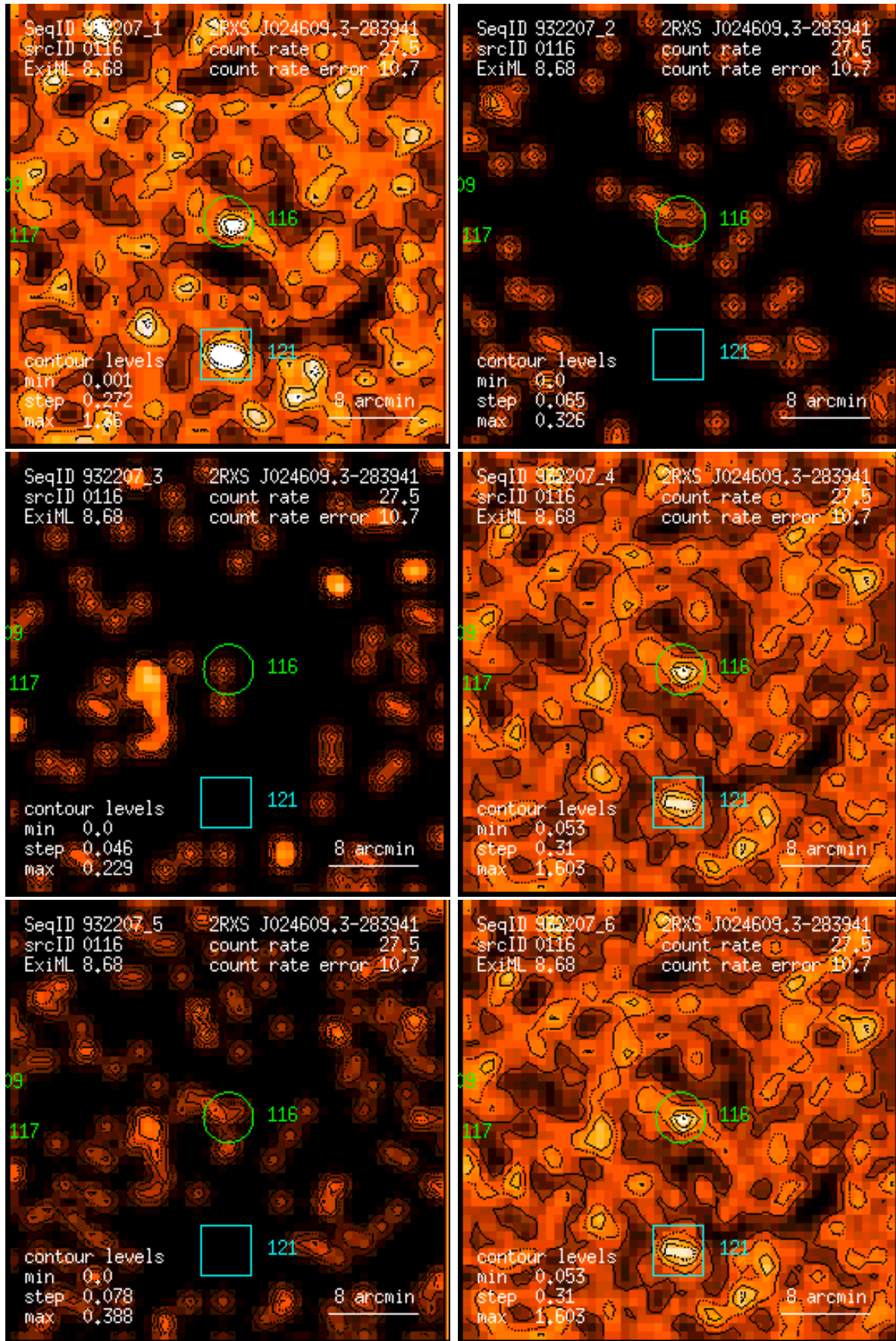
Figure 116: RASS 932207: detection 0116: band rate images, Gaussian filter: (1) PSPC channels 11 – 41, (2) 52 – 90, (3) 91 – 201, (4) 11 – 235, (5) 52 – 201, (6) 11 – 201. Broad band rates in counts/ks. Band rate contour levels in counts/ks/arcmin 2 .
