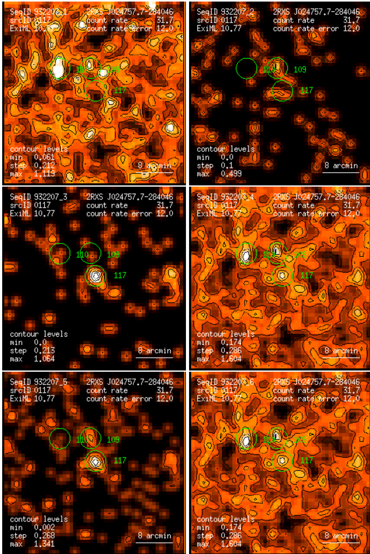
Figure 117: RASS 932207: detection 0117: band rate images, Gaussian filter: (1) PSPC channels 11 – 41, (2) 52 – 90, (3) 91 – 201, (4) 11 – 235, (5) 52 – 201, (6) 11 – 201. Broad band rates in counts/ks. Band rate contour levels in counts/ks/arcmin 2 .
