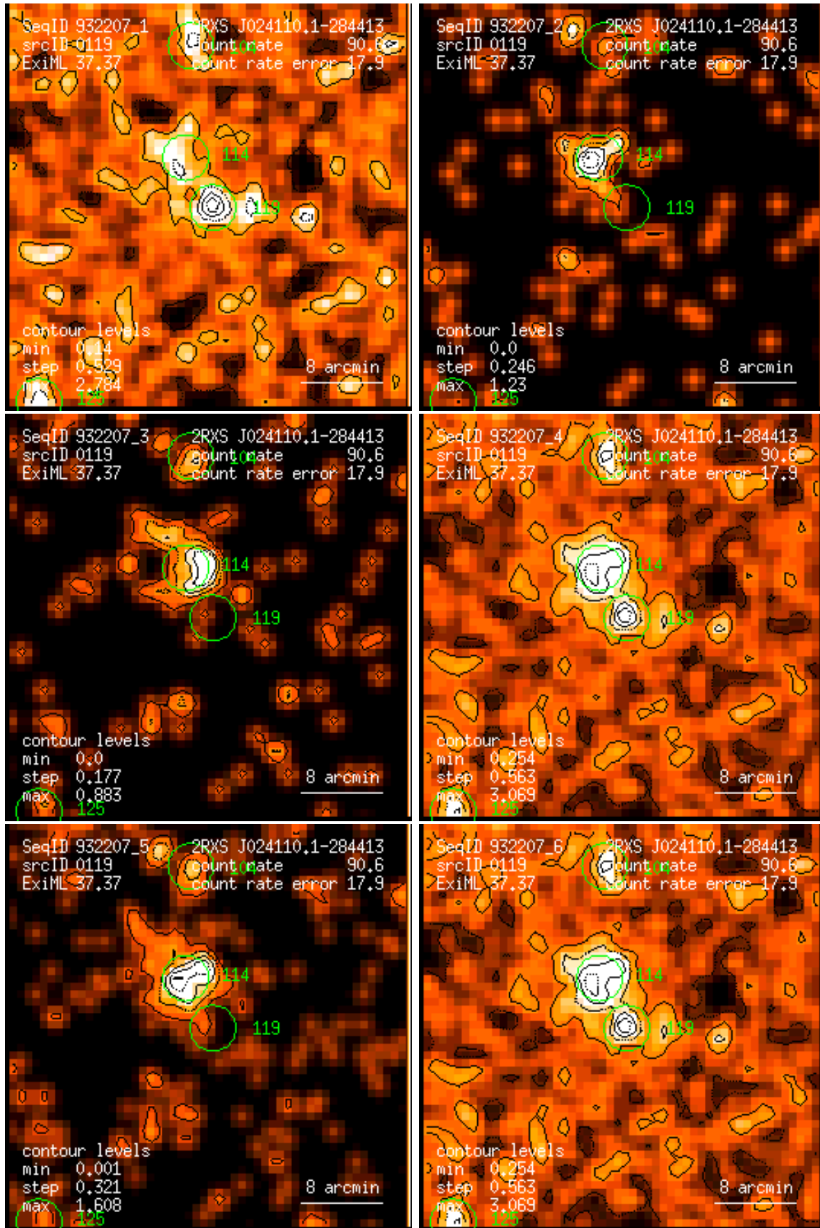
Figure 119: RASS 932207: detection 0119: band rate images, Gaussian filter: (1) PSPC channels 11 – 41, (2) 52 – 90, (3) 91 – 201, (4) 11 – 235, (5) 52 – 201, (6) 11 – 201. Broad band rates in counts/ks. Band rate contour levels in counts/ks/arcmin 2 .
