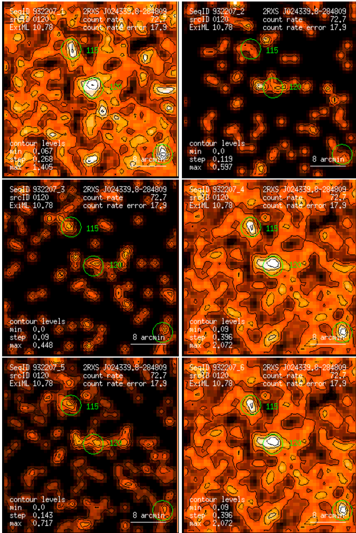
Figure 120: RASS 932207: detection 0120: band rate images, Gaussian filter: (1) PSPC channels 11 – 41, (2) 52 – 90, (3) 91 – 201, (4) 11 – 235, (5) 52 – 201, (6) 11 – 201. Broad band rates in counts/ks. Band rate contour levels in counts/ks/arcmin 2 .
