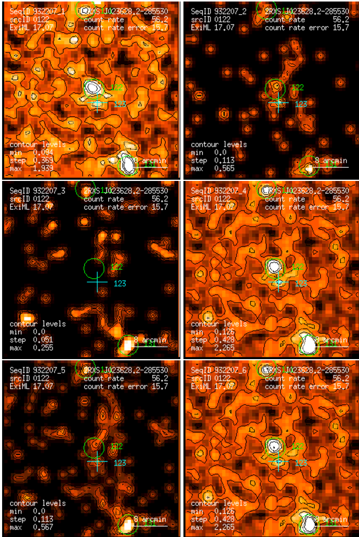
Figure 122: RASS 932207: detection 0122: band rate images, Gaussian filter: (1) PSPC channels 11 – 41, (2) 52 – 90, (3) 91 – 201, (4) 11 – 235, (5) 52 – 201, (6) 11 – 201. Broad band rates in counts/ks. Band rate contour levels in counts/ks/arcmin 2 .
