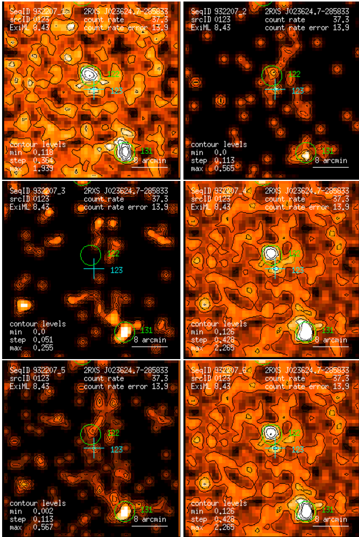
Figure 123: RASS 932207: detection 0123: band rate images, Gaussian filter: (1) PSPC channels 11 – 41, (2) 52 – 90, (3) 91 – 201, (4) 11 – 235, (5) 52 – 201, (6) 11 – 201. Broad band rates in counts/ks. Band rate contour levels in counts/ks/arcmin 2 .
