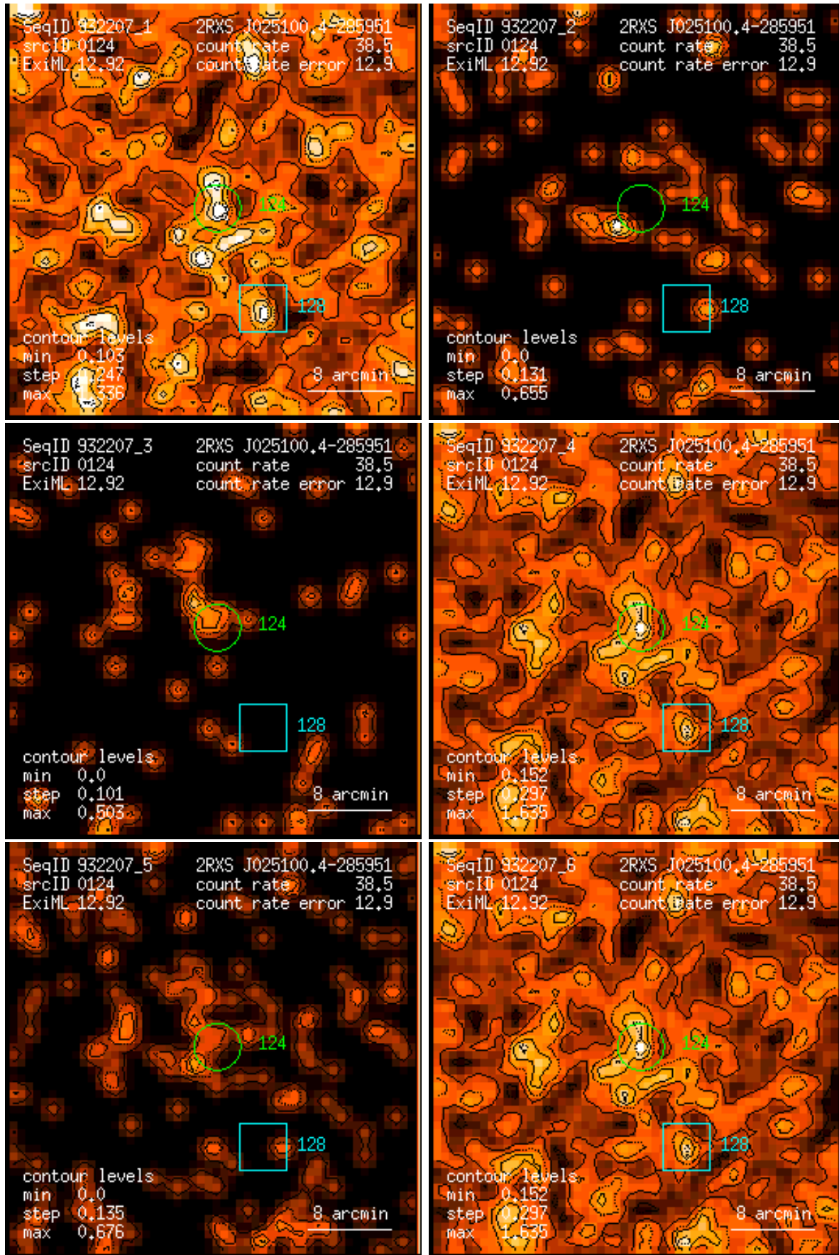
Figure 124: RASS 932207: detection 0124: band rate images, Gaussian filter: (1) PSPC channels 11 – 41, (2) 52 – 90, (3) 91 – 201, (4) 11 – 235, (5) 52 – 201, (6) 11 – 201. Broad band rates in counts/ks. Band rate contour levels in counts/ks/arcmin 2 .
