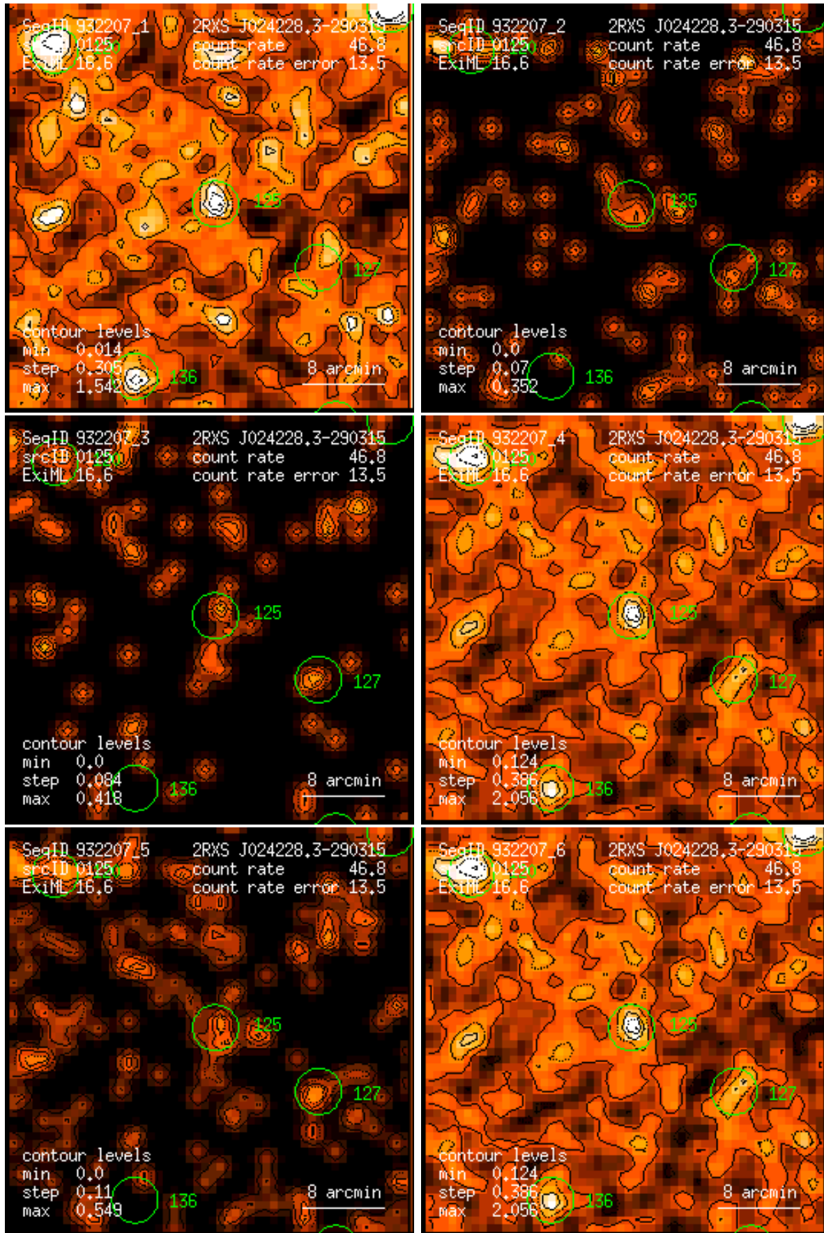
Figure 125: RASS 932207: detection 0125: band rate images, Gaussian filter: (1) PSPC channels 11 – 41, (2) 52 – 90, (3) 91 – 201, (4) 11 – 235, (5) 52 – 201, (6) 11 – 201. Broad band rates in counts/ks. Band rate contour levels in counts/ks/arcmin 2 .
