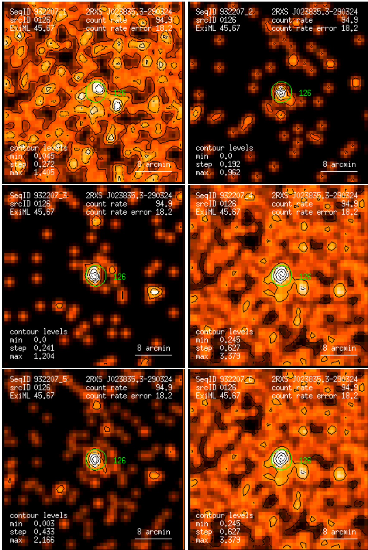
Figure 126: RASS 932207: detection 0126: band rate images, Gaussian filter: (1) PSPC channels 11 – 41, (2) 52 – 90, (3) 91 – 201, (4) 11 – 235, (5) 52 – 201, (6) 11 – 201. Broad band rates in counts/ks. Band rate contour levels in counts/ks/arcmin 2 .
