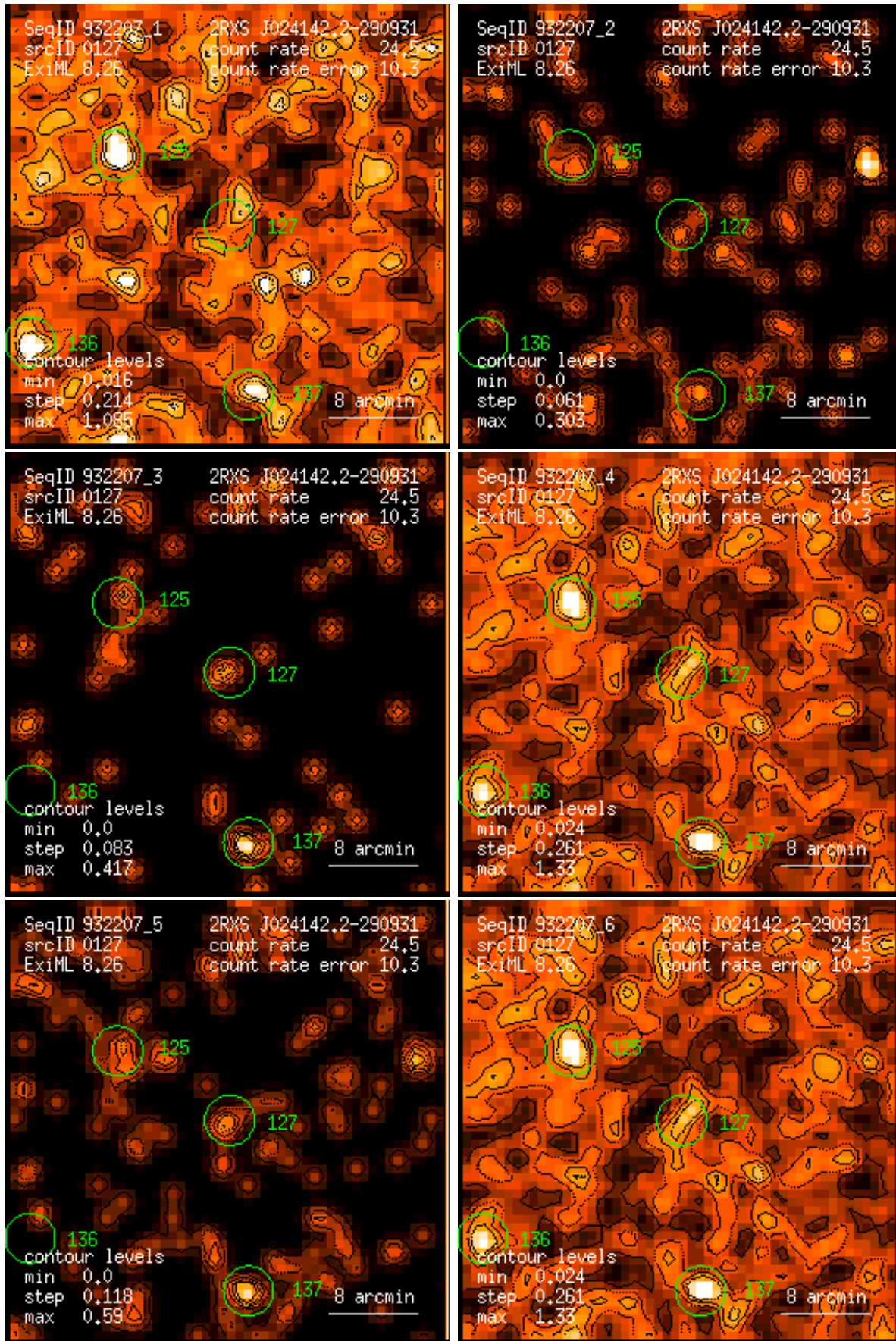
Figure 127: RASS 932207: detection 0127: band rate images, Gaussian filter: (1) PSPC channels 11 – 41, (2) 52 – 90, (3) 91 – 201, (4) 11 – 235, (5) 52 – 201, (6) 11 – 201. Broad band rates in counts/ks. Band rate contour levels in counts/ks/arcmin 2 .
