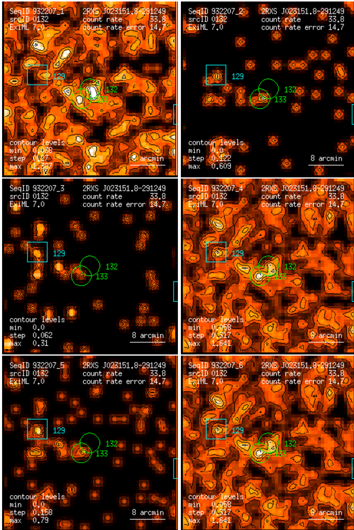
Figure 132: RASS 932207: detection 0132: band rate images, Gaussian filter: (1) PSPC channels 11 – 41, (2) 52 – 90, (3) 91 – 201, (4) 11 – 235, (5) 52 – 201, (6) 11 – 201. Broad band rates in counts/ks. Band rate contour levels in counts/ks/arcmin 2 .
