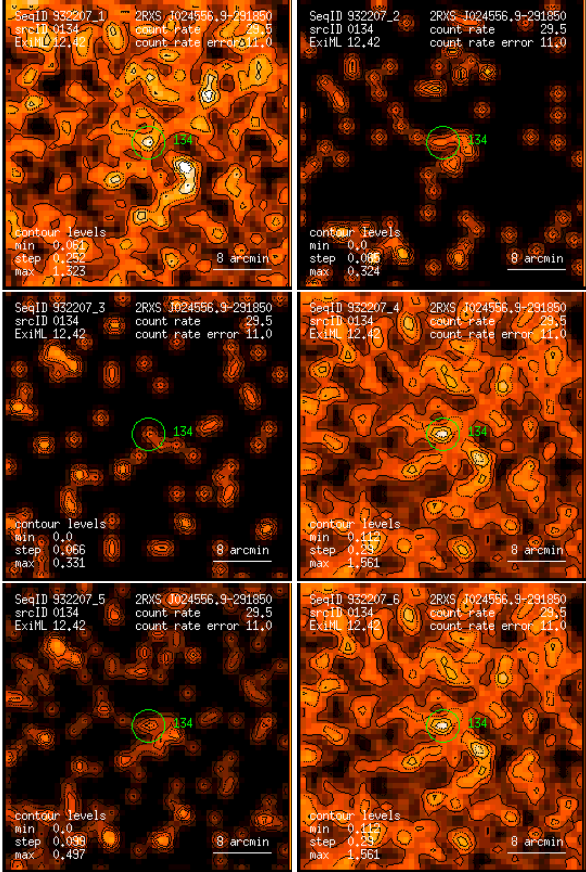
Figure 134: RASS 932207: detection 0134: band rate images, Gaussian filter: (1) PSPC channels 11 – 41, (2) 52 – 90, (3) 91 – 201, (4) 11 – 235, (5) 52 – 201, (6) 11 – 201. Broad band rates in counts/ks. Band rate contour levels in counts/ks/arcmin 2 .
