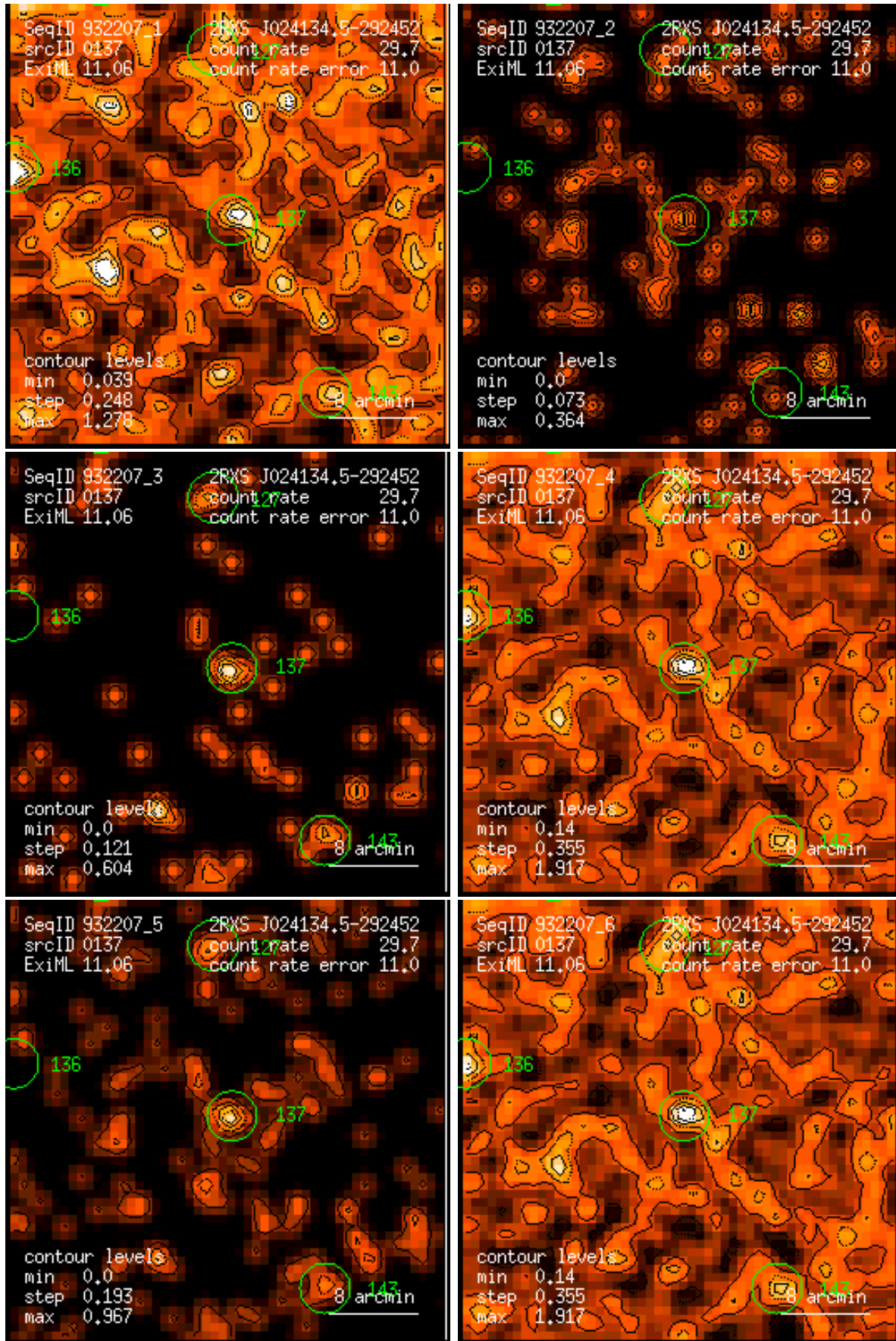
Figure 137: RASS 932207: detection 0137: band rate images, Gaussian filter: (1) PSPC channels 11 – 41, (2) 52 – 90, (3) 91 – 201, (4) 11 – 235, (5) 52 – 201, (6) 11 – 201. Broad band rates in counts/ks. Band rate contour levels in counts/ks/arcmin 2 .
