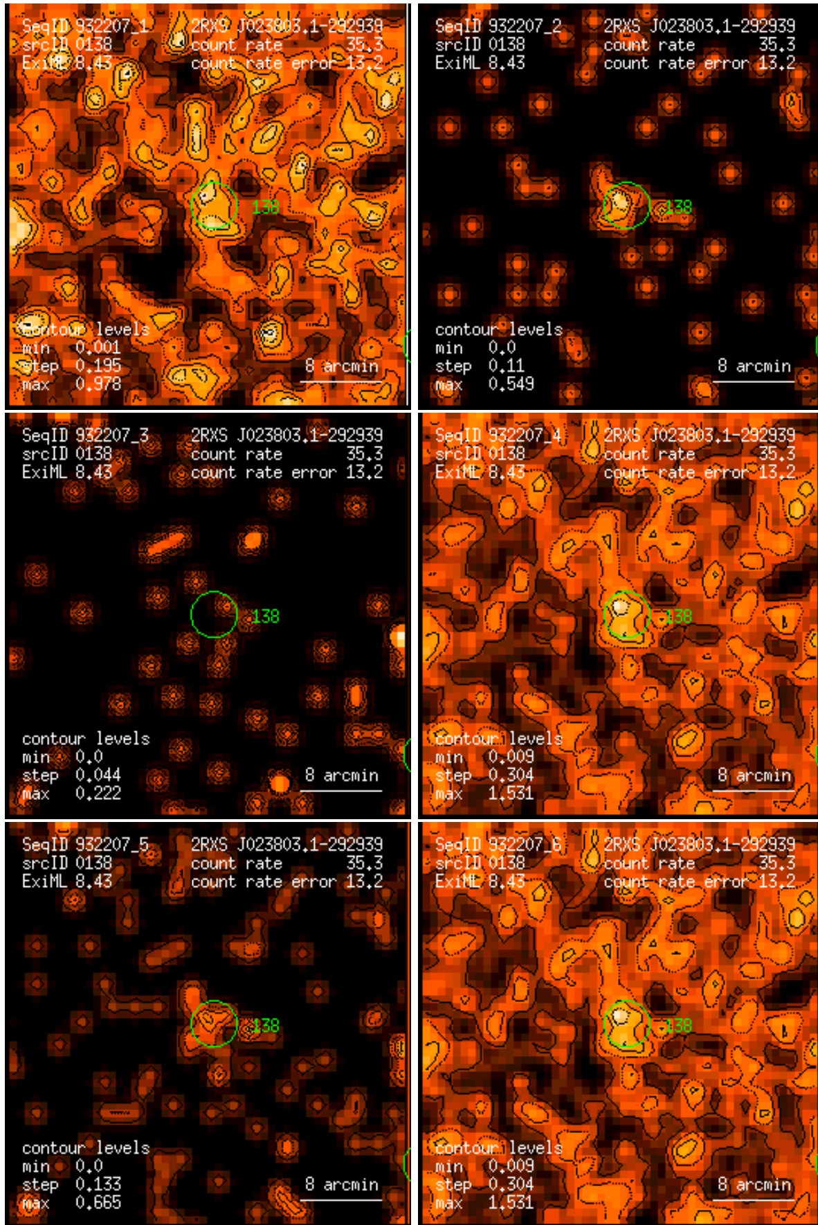
Figure 138: RASS 932207: detection 0138: band rate images, Gaussian filter: (1) PSPC channels 11 – 41, (2) 52 – 90, (3) 91 – 201, (4) 11 – 235, (5) 52 – 201, (6) 11 – 201. Broad band rates in counts/ks. Band rate contour levels in counts/ks/arcmin 2 .
