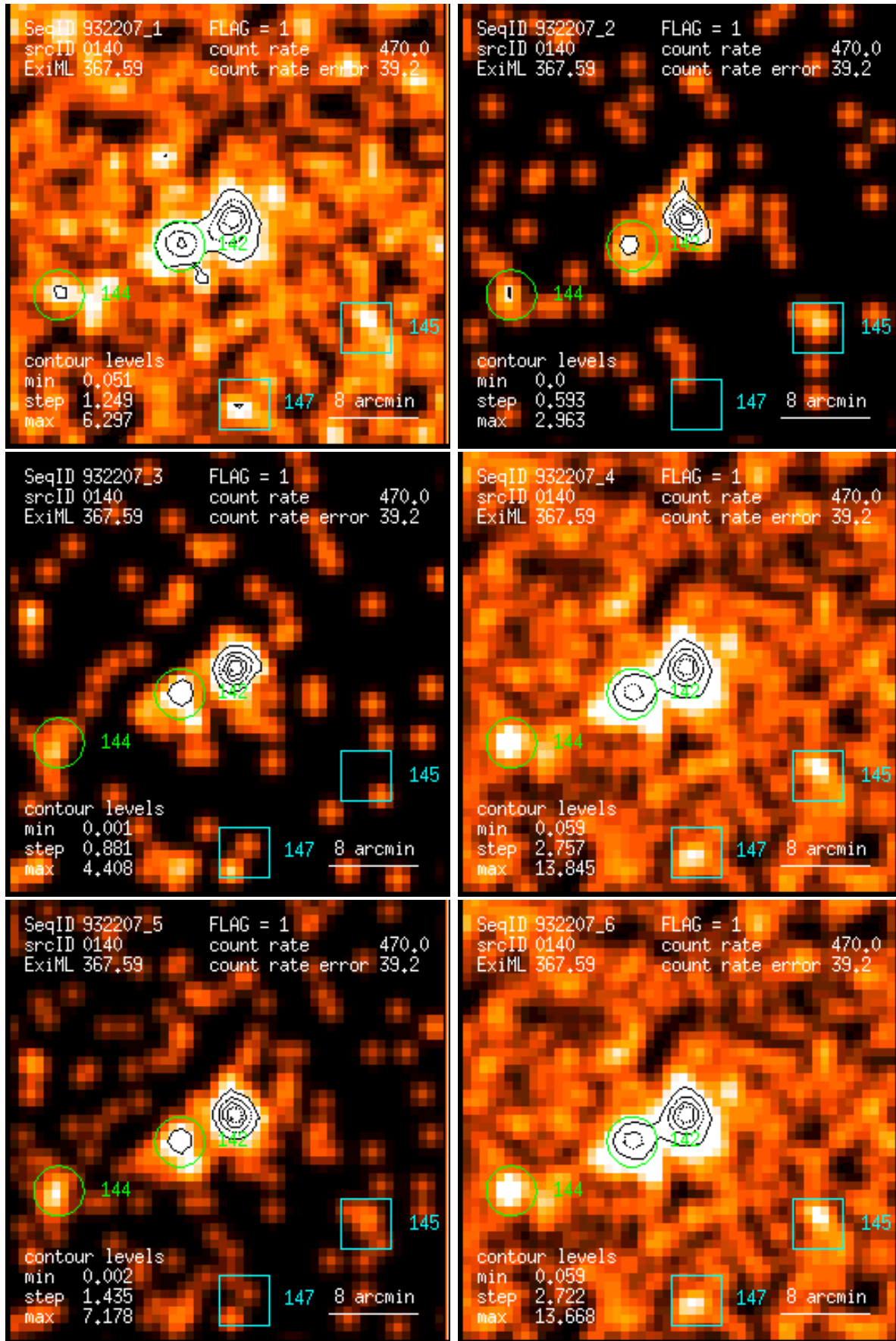
Figure 140: RASS 932207: detection 0140: band rate images, Gaussian filter: (1) PSPC channels 11 – 41, (2) 52 – 90, (3) 91 – 201, (4) 11 – 235, (5) 52 – 201, (6) 11 – 201. Broad band rates in counts/ks. Band rate contour levels in counts/ks/arcmin 2 .
