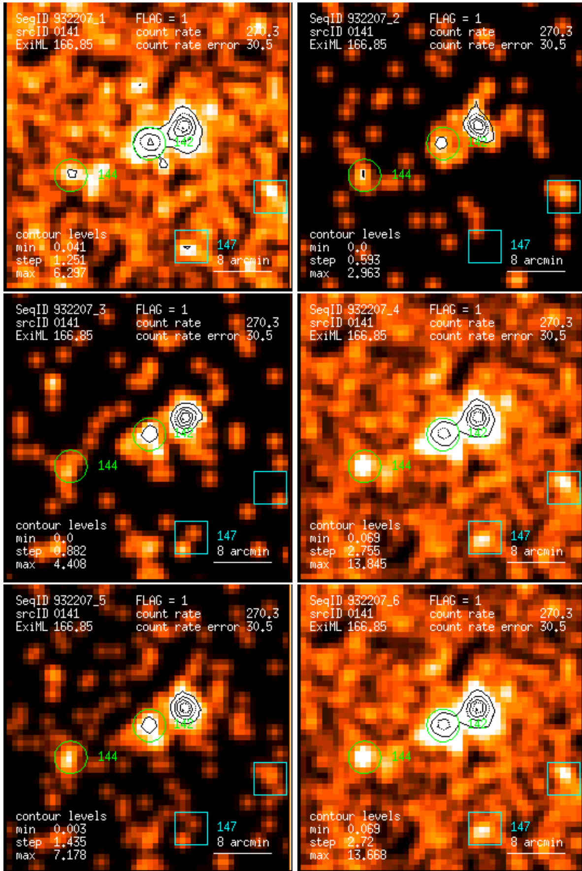
Figure 141: RASS 932207: detection 0141: band rate images, Gaussian filter: (1) PSPC channels 11 – 41, (2) 52 – 90, (3) 91 – 201, (4) 11 – 235, (5) 52 – 201, (6) 11 – 201. Broad band rates in counts/ks. Band rate contour levels in counts/ks/arcmin 2 .
