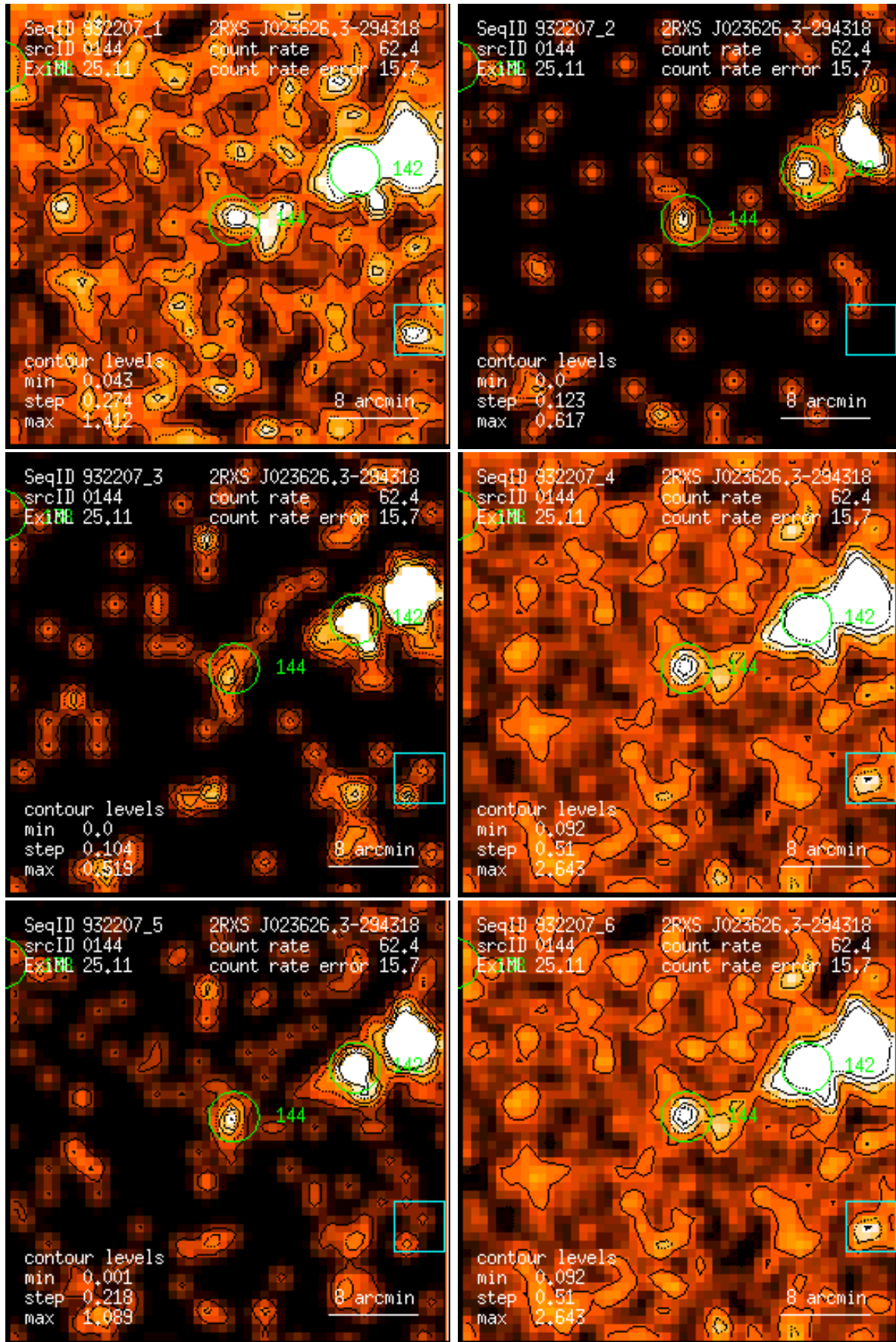
Figure 144: RASS 932207: detection 0144: band rate images, Gaussian filter: (1) PSPC channels 11 – 41, (2) 52 – 90, (3) 91 – 201, (4) 11 – 235, (5) 52 – 201, (6) 11 – 201. Broad band rates in counts/ks. Band rate contour levels in counts/ks/arcmin 2 .
