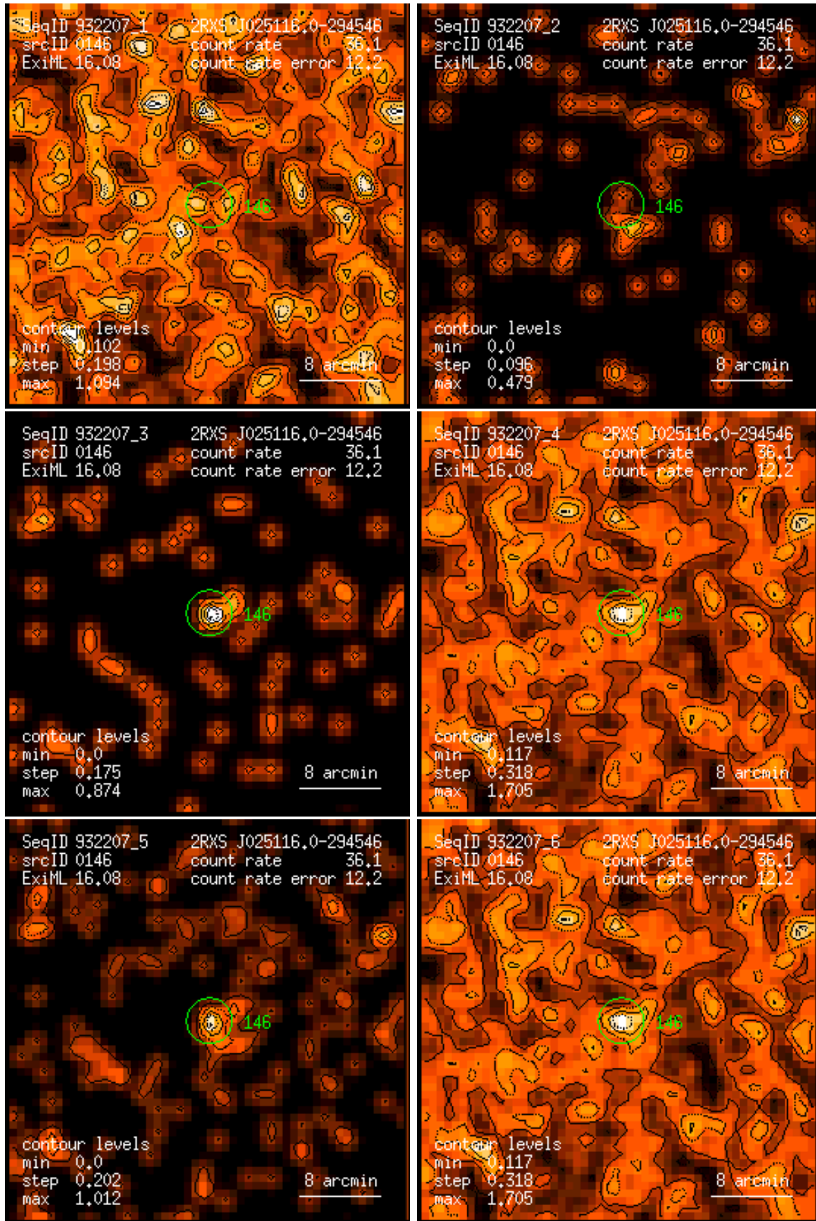
Figure 146: RASS 932207: detection 0146: band rate images, Gaussian filter: (1) PSPC channels 11 – 41, (2) 52 – 90, (3) 91 – 201, (4) 11 – 235, (5) 52 – 201, (6) 11 – 201. Broad band rates in counts/ks. Band rate contour levels in counts/ks/arcmin 2 .
