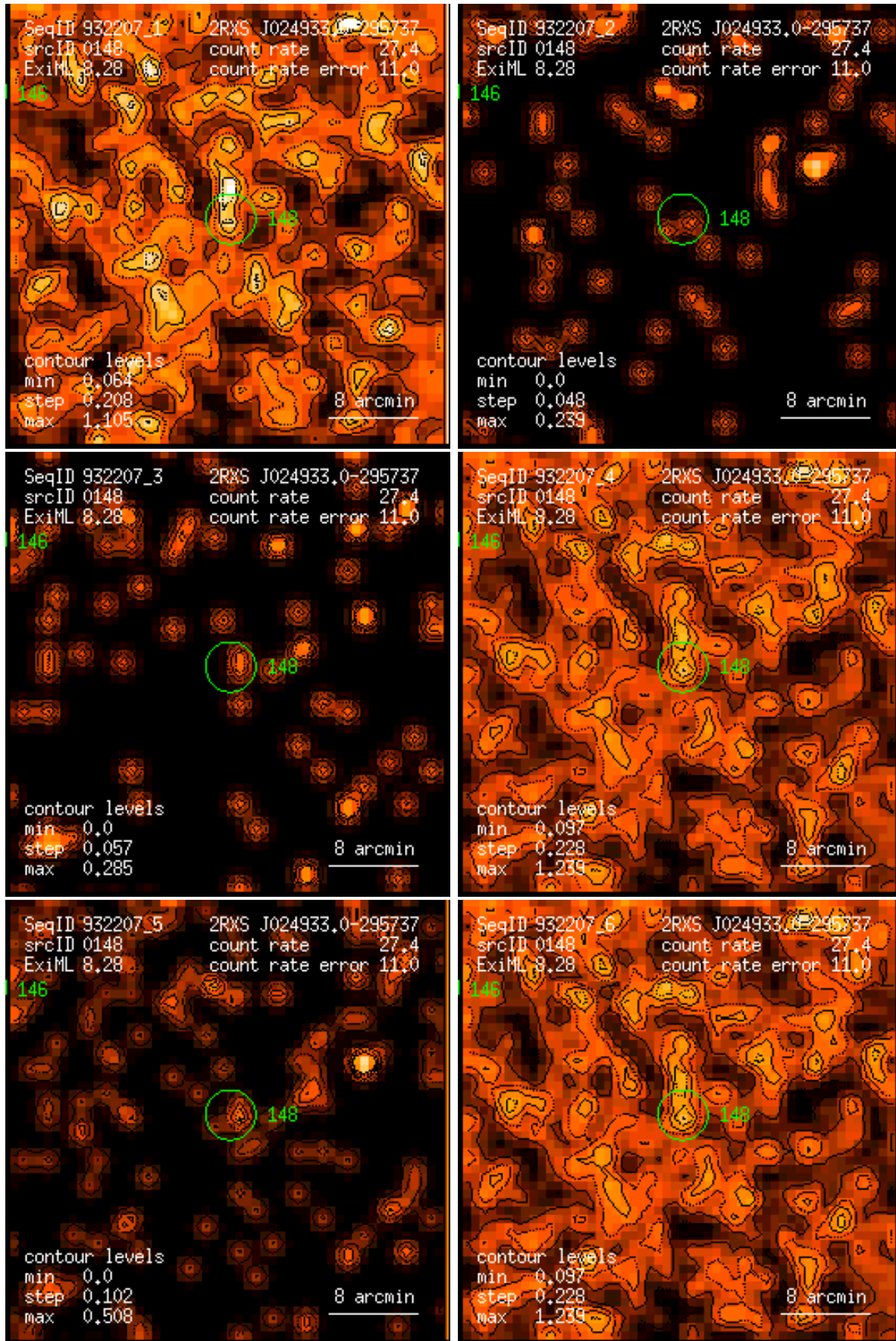
Figure 148: RASS 932207: detection 0148: band rate images, Gaussian filter: (1) PSPC channels 11 – 41, (2) 52 – 90, (3) 91 – 201, (4) 11 – 235, (5) 52 – 201, (6) 11 – 201. Broad band rates in counts/ks. Band rate contour levels in counts/ks/arcmin 2 .
