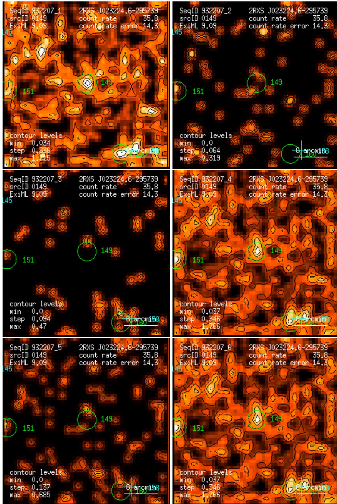
Figure 149: RASS 932207: detection 0149: band rate images, Gaussian filter: (1) PSPC channels 11 – 41, (2) 52 – 90, (3) 91 – 201, (4) 11 – 235, (5) 52 – 201, (6) 11 – 201. Broad band rates in counts/ks. Band rate contour levels in counts/ks/arcmin 2 .
