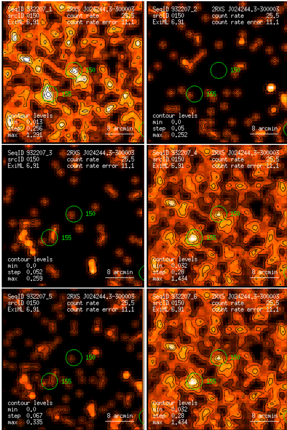
Figure 150: RASS 932207: detection 0150: band rate images, Gaussian filter: (1) PSPC channels 11 – 41, (2) 52 – 90, (3) 91 – 201, (4) 11 – 235, (5) 52 – 201, (6) 11 – 201. Broad band rates in counts/ks. Band rate contour levels in counts/ks/arcmin 2 .
