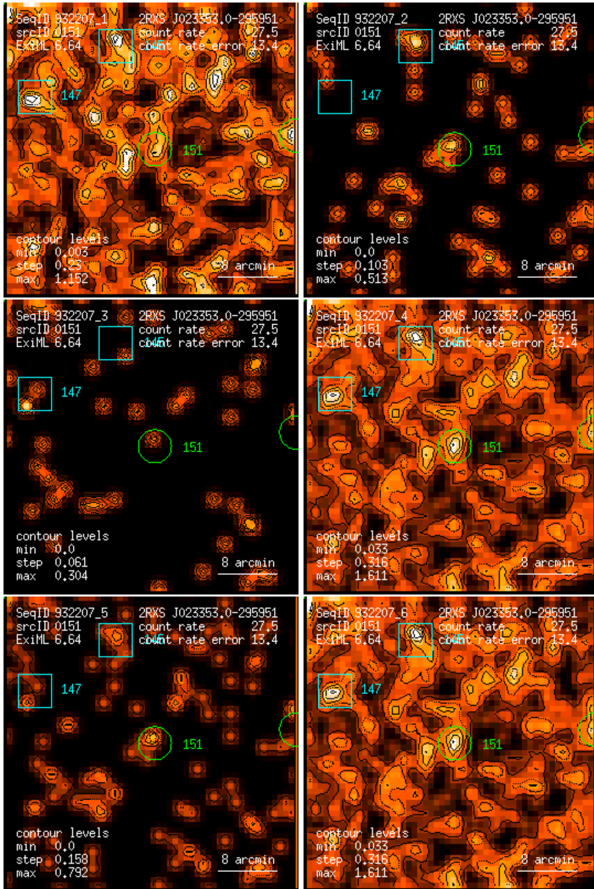
Figure 151: RASS 932207: detection 0151: band rate images, Gaussian filter: (1) PSPC channels 11 – 41, (2) 52 – 90, (3) 91 – 201, (4) 11 – 235, (5) 52 – 201, (6) 11 – 201. Broad band rates in counts/ks. Band rate contour levels in counts/ks/arcmin 2 .
