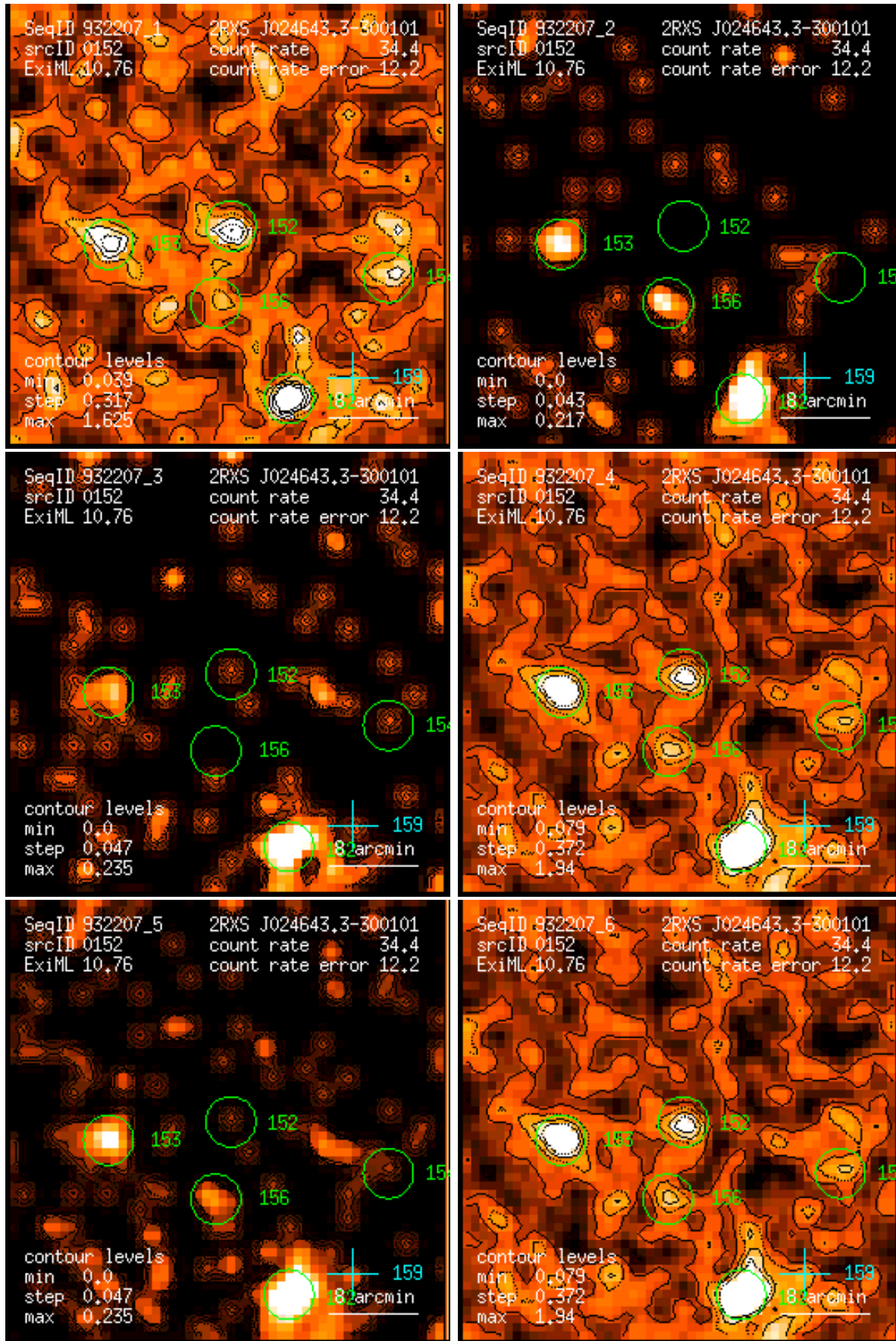
Figure 152: RASS 932207: detection 0152: band rate images, Gaussian filter: (1) PSPC channels 11 – 41, (2) 52 – 90, (3) 91 – 201, (4) 11 – 235, (5) 52 – 201, (6) 11 – 201. Broad band rates in counts/ks. Band rate contour levels in counts/ks/arcmin 2 .
