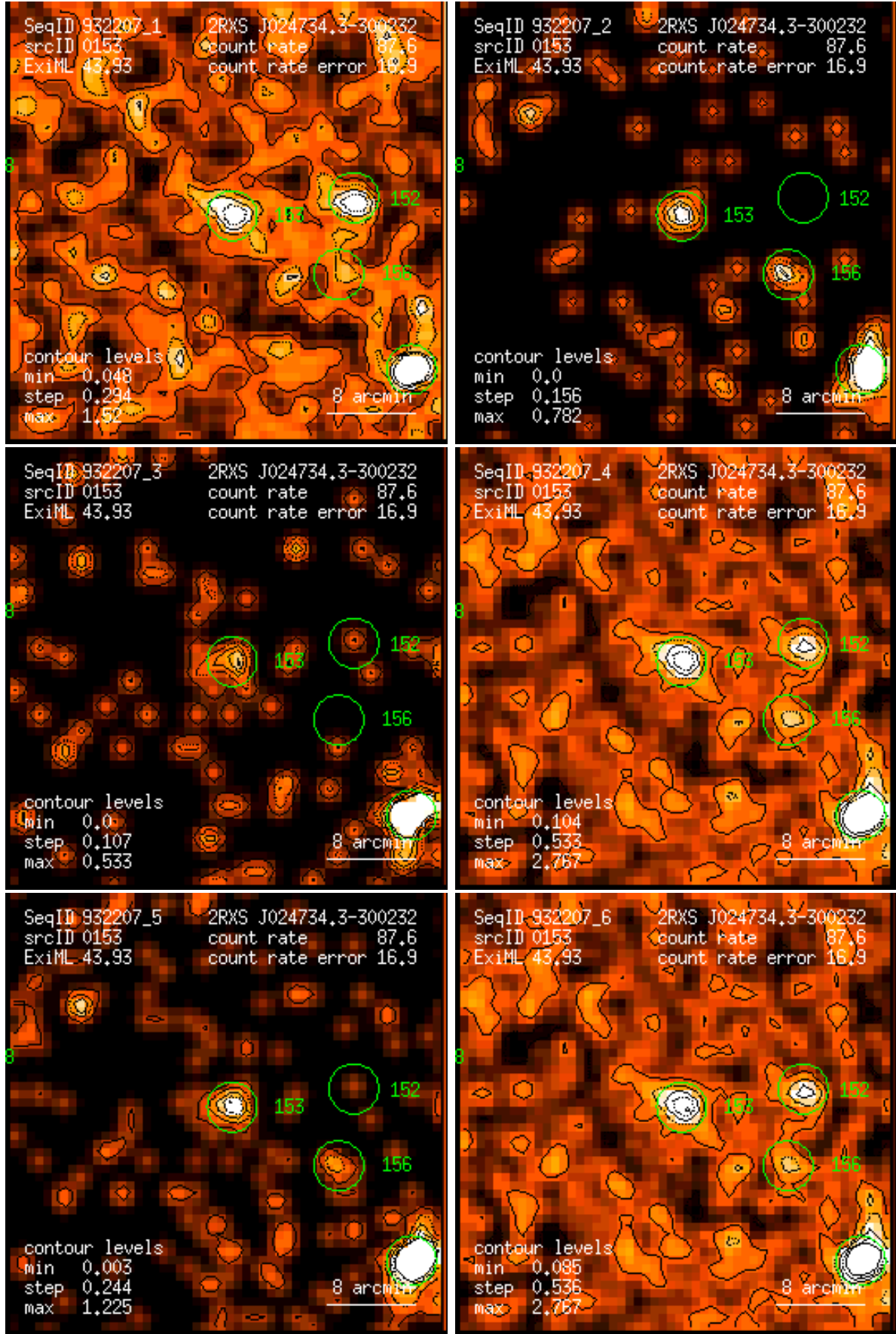
Figure 153: RASS 932207: detection 0153: band rate images, Gaussian filter: (1) PSPC channels 11 – 41, (2) 52 – 90, (3) 91 – 201, (4) 11 – 235, (5) 52 – 201, (6) 11 – 201. Broad band rates in counts/ks. Band rate contour levels in counts/ks/arcmin 2 .
