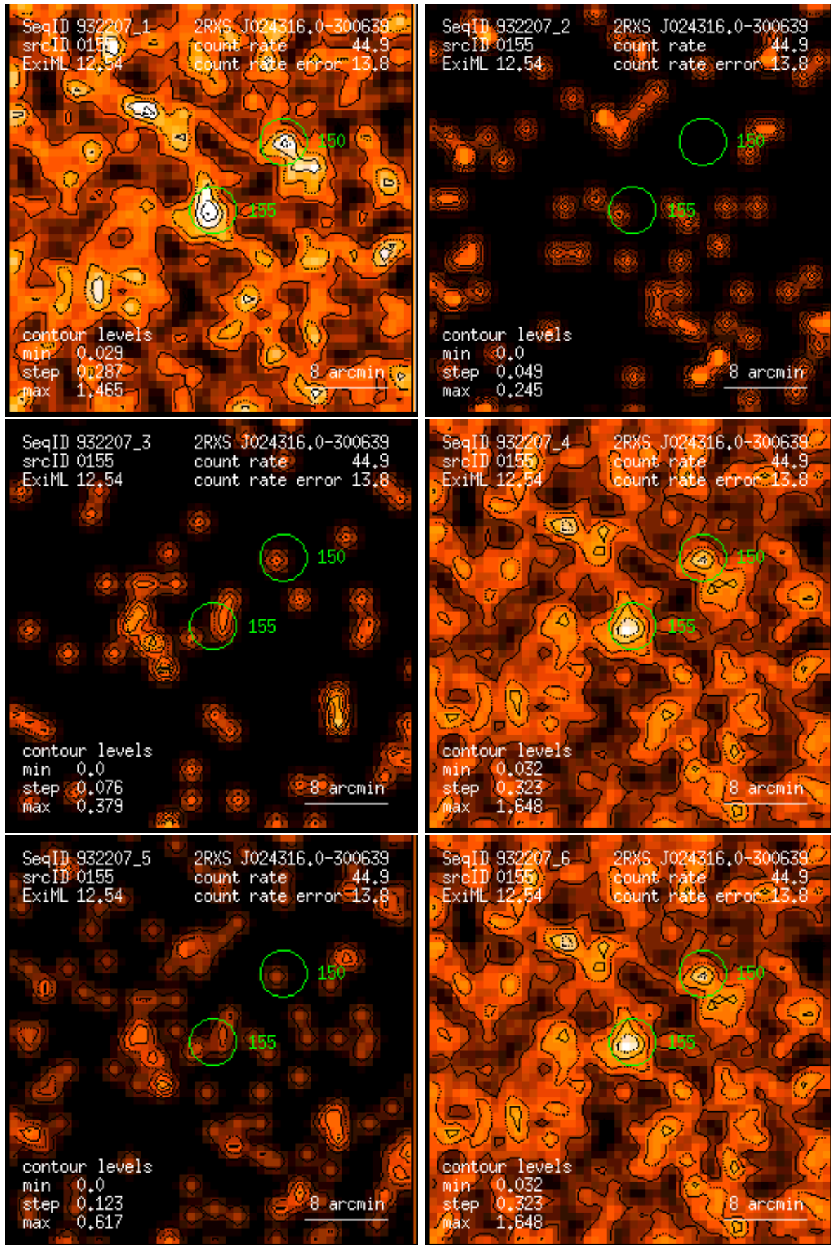
Figure 155: RASS 932207: detection 0155: band rate images, Gaussian filter: (1) PSPC channels 11 – 41, (2) 52 – 90, (3) 91 – 201, (4) 11 – 235, (5) 52 – 201, (6) 11 – 201. Broad band rates in counts/ks. Band rate contour levels in counts/ks/arcmin 2 .
