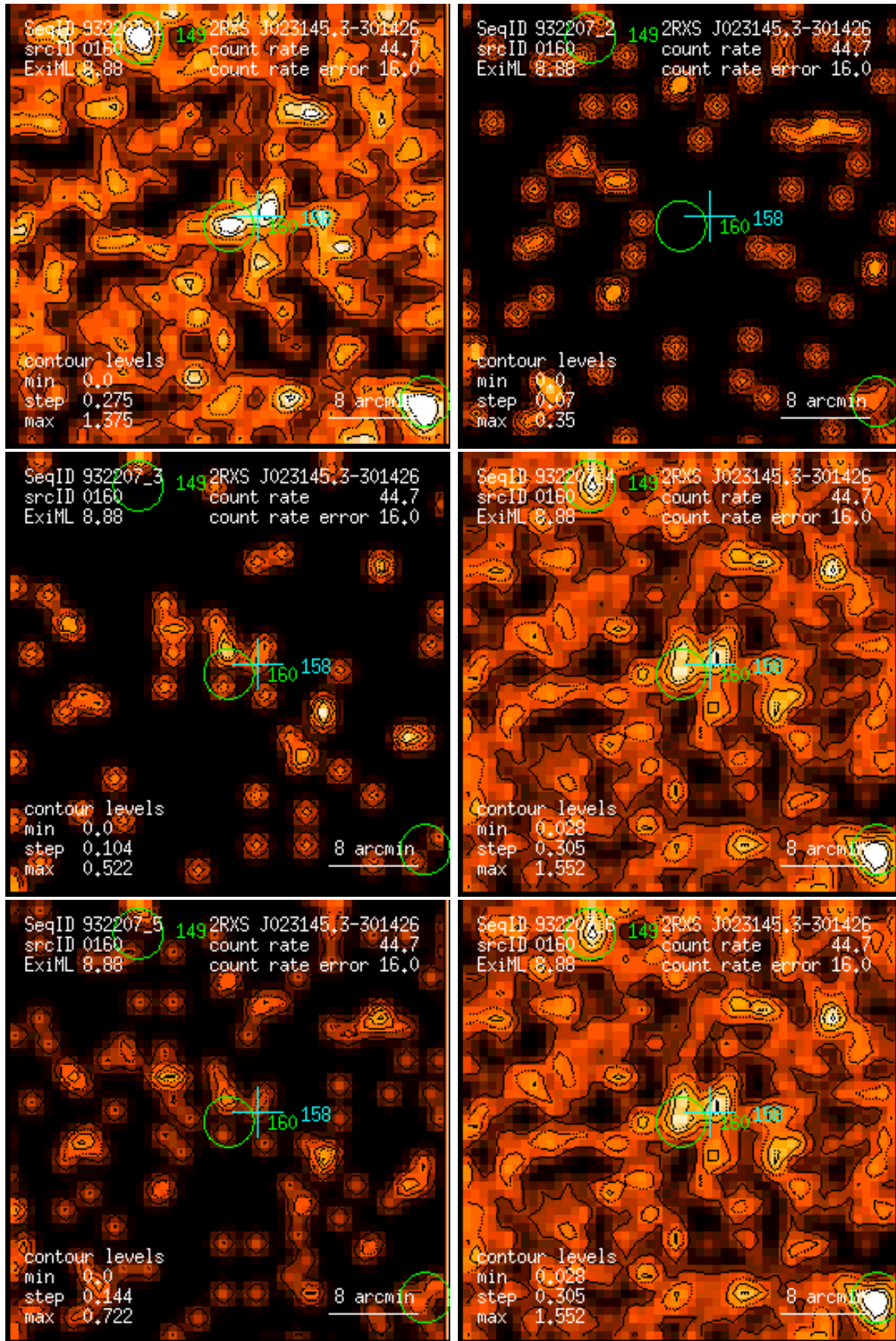
Figure 160: RASS 932207: detection 0160: band rate images, Gaussian filter: (1) PSPC channels 11 – 41, (2) 52 – 90, (3) 91 – 201, (4) 11 – 235, (5) 52 – 201, (6) 11 – 201. Broad band rates in counts/ks. Band rate contour levels in counts/ks/arcmin 2 .
