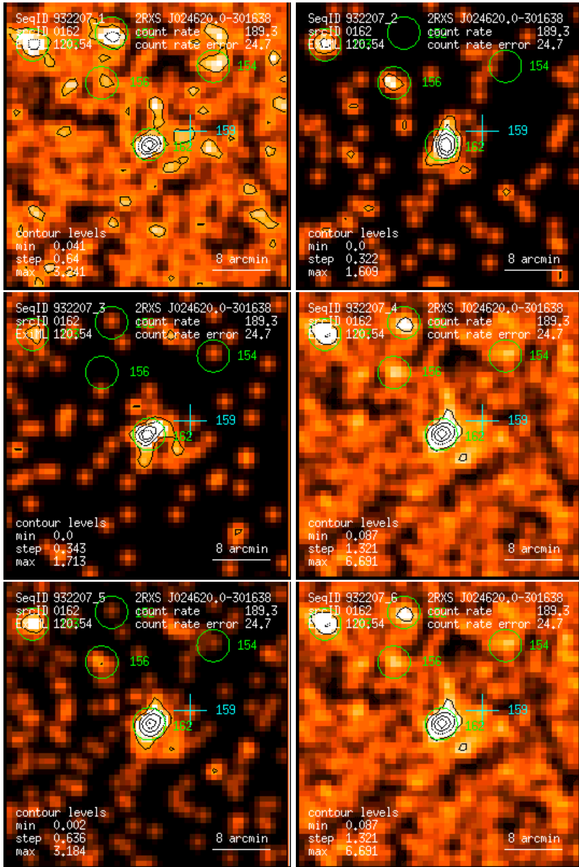
Figure 162: RASS 932207: detection 0162: band rate images, Gaussian filter: (1) PSPC channels 11 – 41, (2) 52 – 90, (3) 91 – 201, (4) 11 – 235, (5) 52 – 201, (6) 11 – 201. Broad band rates in counts/ks. Band rate contour levels in counts/ks/arcmin 2 .
