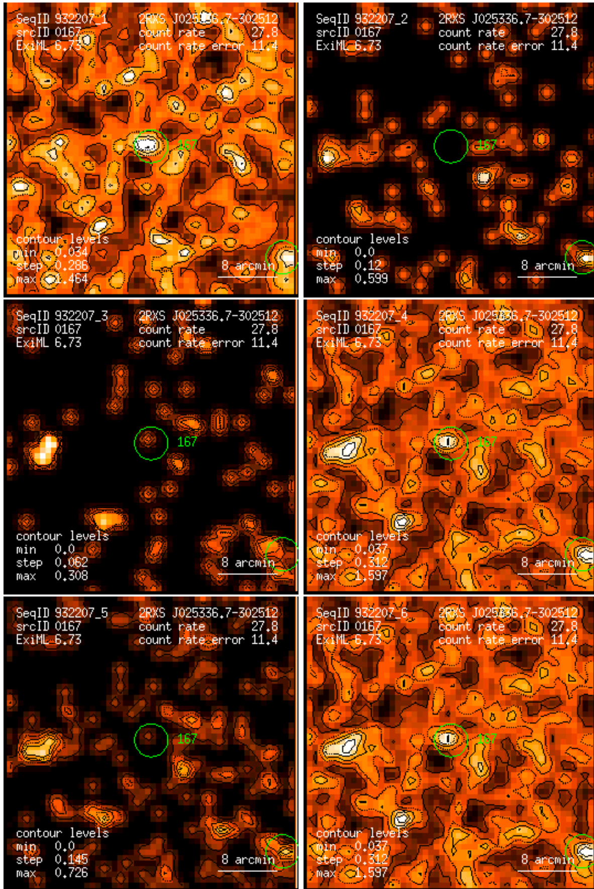
Figure 167: RASS 932207: detection 0167: band rate images, Gaussian filter: (1) PSPC channels 11 – 41, (2) 52 – 90, (3) 91 – 201, (4) 11 – 235, (5) 52 – 201, (6) 11 – 201. Broad band rates in counts/ks. Band rate contour levels in counts/ks/arcmin 2 .
