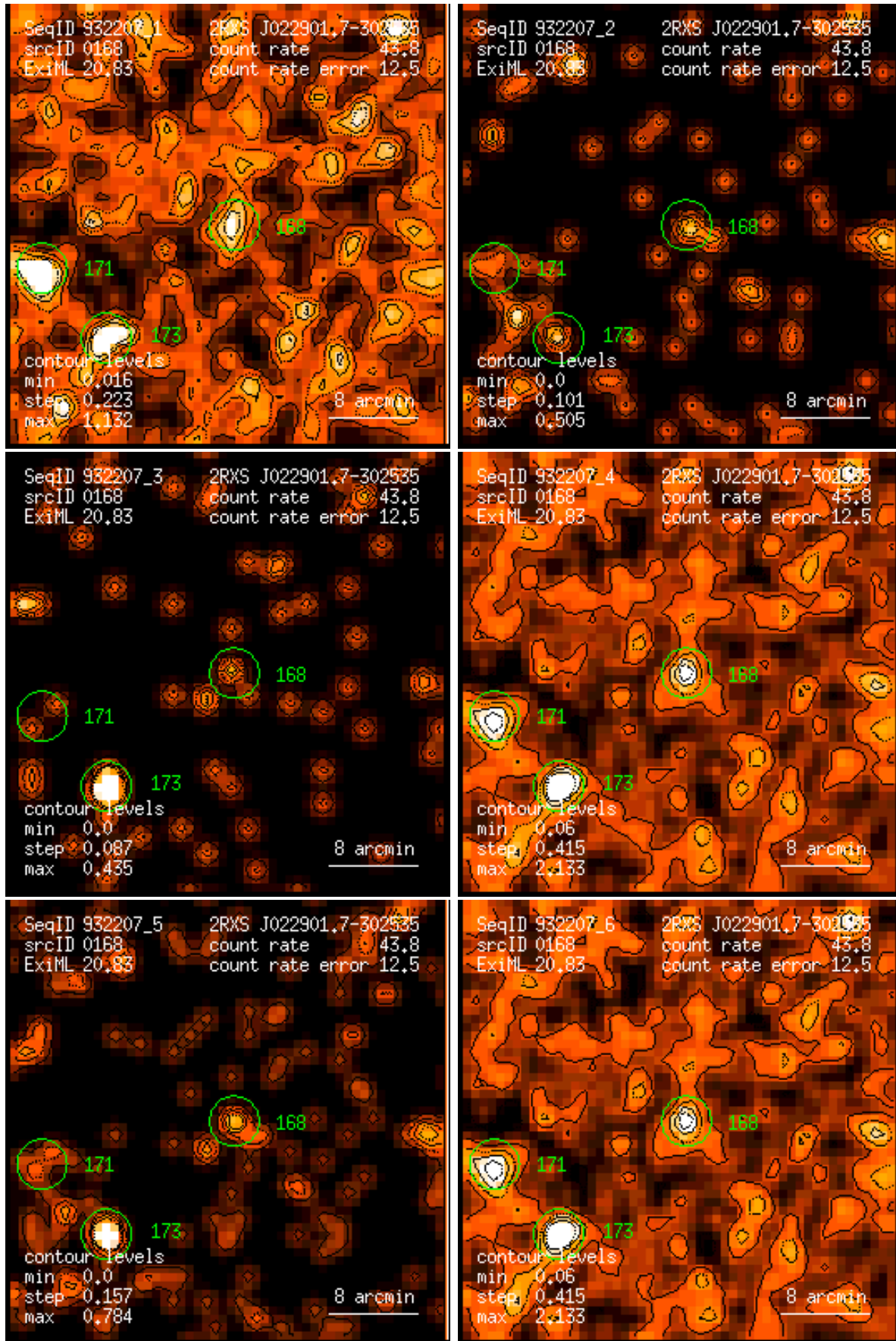
Figure 168: RASS 932207: detection 0168: band rate images, Gaussian filter: (1) PSPC channels 11 – 41, (2) 52 – 90, (3) 91 – 201, (4) 11 – 235, (5) 52 – 201, (6) 11 – 201. Broad band rates in counts/ks. Band rate contour levels in counts/ks/arcmin 2 .
