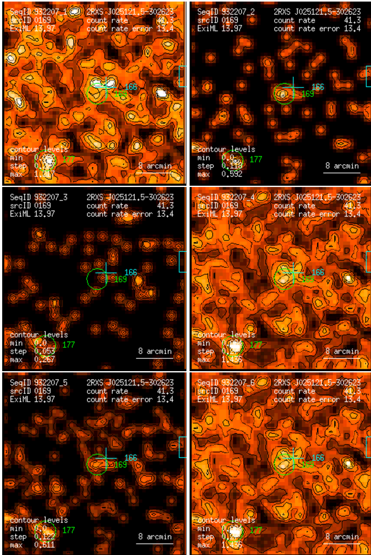
Figure 169: RASS 932207: detection 0169: band rate images, Gaussian filter: (1) PSPC channels 11 – 41, (2) 52 – 90, (3) 91 – 201, (4) 11 – 235, (5) 52 – 201, (6) 11 – 201. Broad band rates in counts/ks. Band rate contour levels in counts/ks/arcmin 2 .
