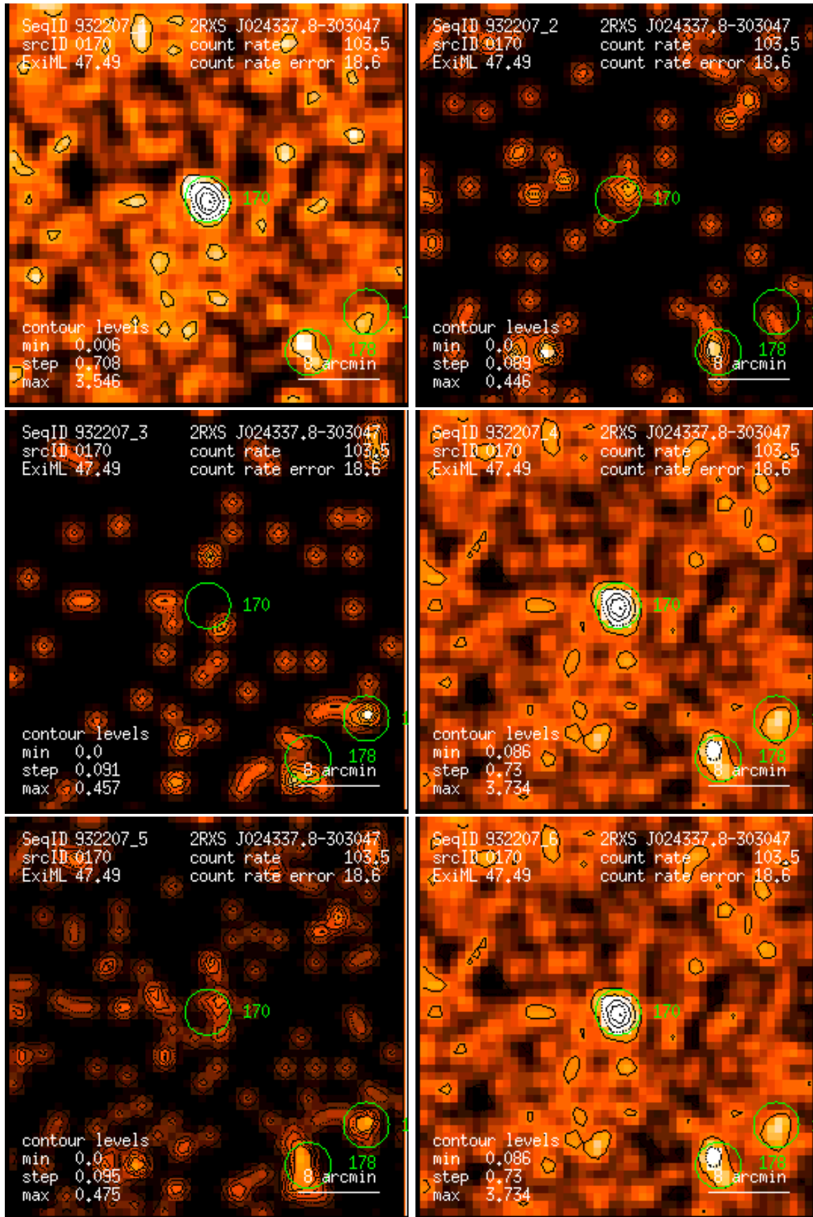
Figure 170: RASS 932207: detection 0170: band rate images, Gaussian filter: (1) PSPC channels 11 – 41, (2) 52 – 90, (3) 91 – 201, (4) 11 – 235, (5) 52 – 201, (6) 11 – 201. Broad band rates in counts/ks. Band rate contour levels in counts/ks/arcmin 2 .
