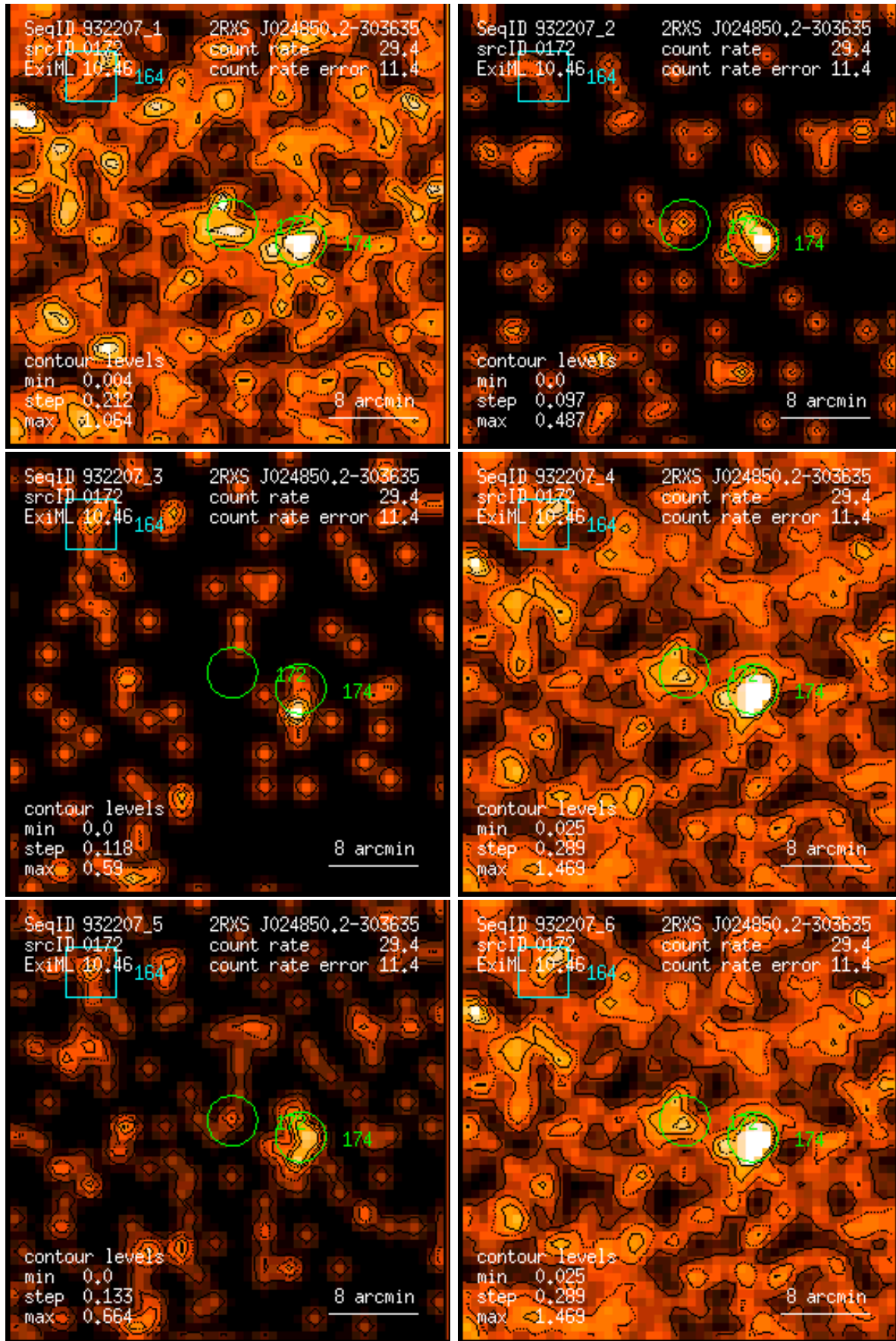
Figure 172: RASS 932207: detection 0172: band rate images, Gaussian filter: (1) PSPC channels 11 – 41, (2) 52 – 90, (3) 91 – 201, (4) 11 – 235, (5) 52 – 201, (6) 11 – 201. Broad band rates in counts/ks. Band rate contour levels in counts/ks/arcmin 2 .
