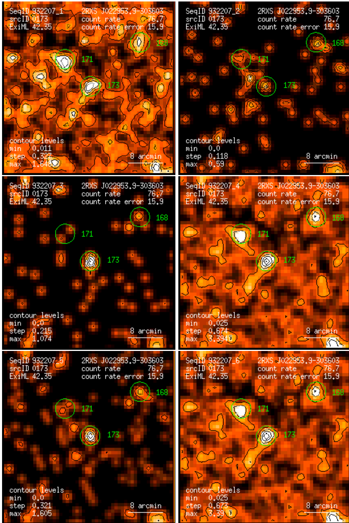
Figure 173: RASS 932207: detection 0173: band rate images, Gaussian filter: (1) PSPC channels 11 – 41, (2) 52 – 90, (3) 91 – 201, (4) 11 – 235, (5) 52 – 201, (6) 11 – 201. Broad band rates in counts/ks. Band rate contour levels in counts/ks/arcmin 2 .
