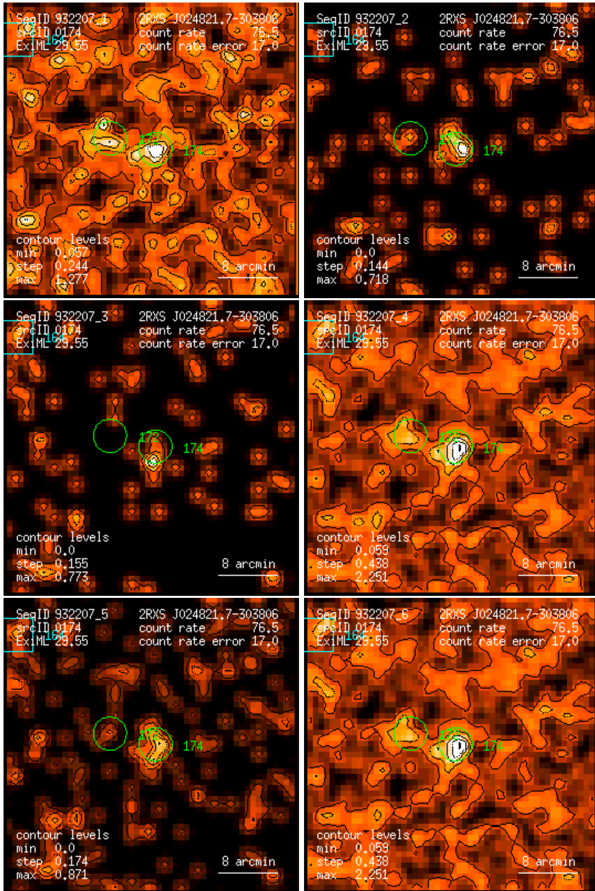
Figure 174: RASS 932207: detection 0174: band rate images, Gaussian filter: (1) PSPC channels 11 – 41, (2) 52 – 90, (3) 91 – 201, (4) 11 – 235, (5) 52 – 201, (6) 11 – 201. Broad band rates in counts/ks. Band rate contour levels in counts/ks/arcmin 2 .
