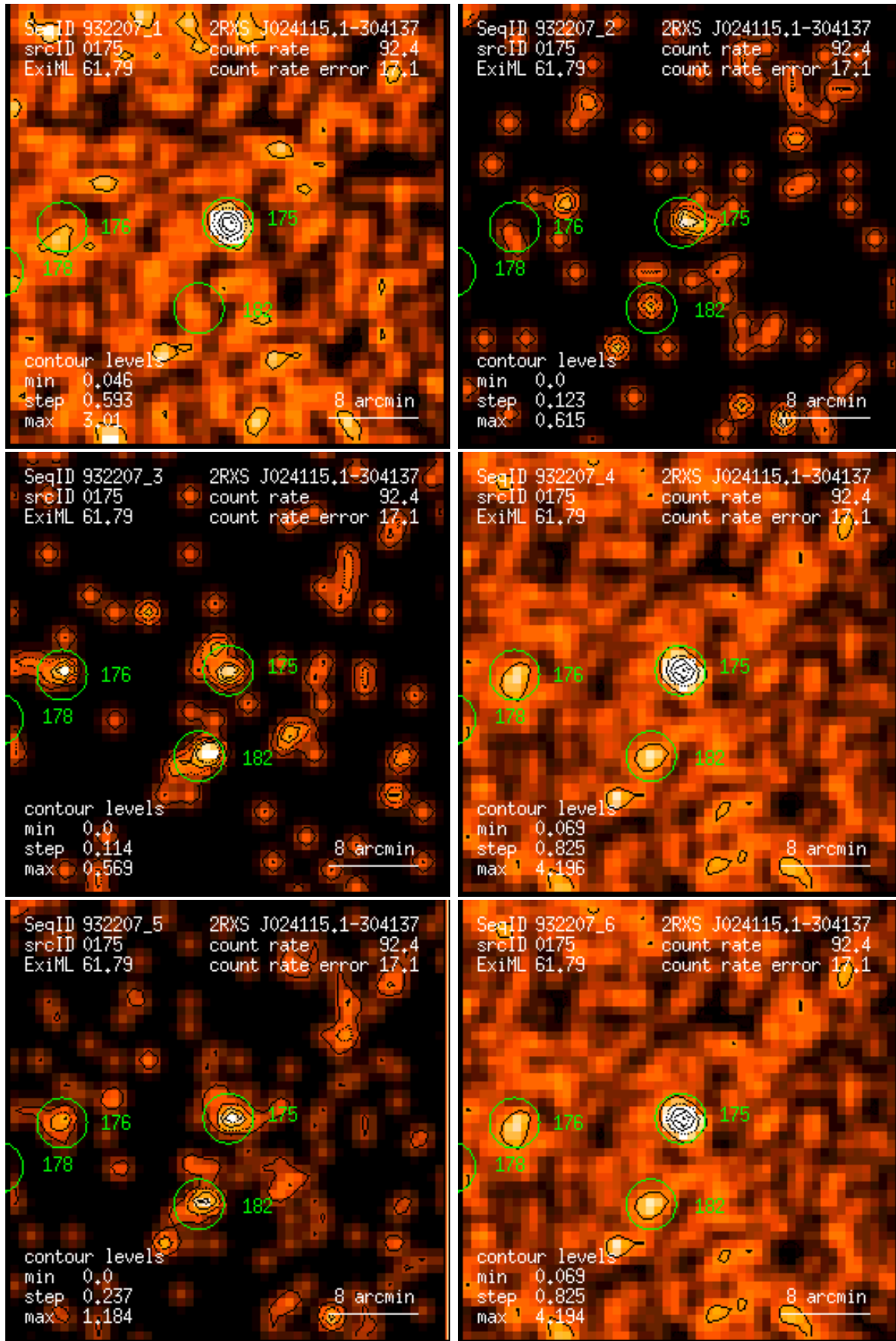
Figure 175: RASS 932207: detection 0175: band rate images, Gaussian filter: (1) PSPC channels 11 – 41, (2) 52 – 90, (3) 91 – 201, (4) 11 – 235, (5) 52 – 201, (6) 11 – 201. Broad band rates in counts/ks. Band rate contour levels in counts/ks/arcmin 2 .
