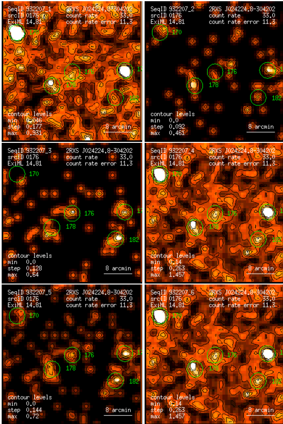
Figure 176: RASS 932207: detection 0176: band rate images, Gaussian filter: (1) PSPC channels 11 – 41, (2) 52 – 90, (3) 91 – 201, (4) 11 – 235, (5) 52 – 201, (6) 11 – 201. Broad band rates in counts/ks. Band rate contour levels in counts/ks/arcmin 2 .
