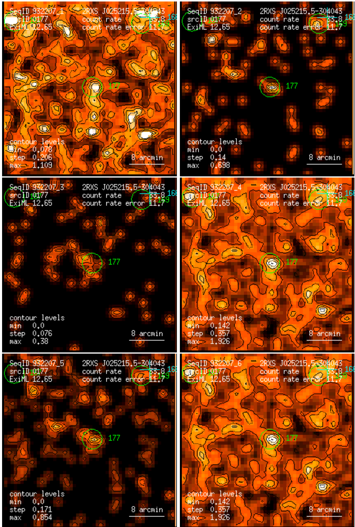
Figure 177: RASS 932207: detection 0177: band rate images, Gaussian filter: (1) PSPC channels 11 – 41, (2) 52 – 90, (3) 91 – 201, (4) 11 – 235, (5) 52 – 201, (6) 11 – 201. Broad band rates in counts/ks. Band rate contour levels in counts/ks/arcmin 2 .
