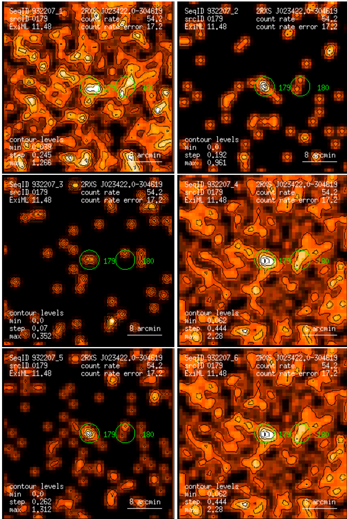
Figure 179: RASS 932207: detection 0179: band rate images, Gaussian filter: (1) PSPC channels 11 – 41, (2) 52 – 90, (3) 91 – 201, (4) 11 – 235, (5) 52 – 201, (6) 11 – 201. Broad band rates in counts/ks. Band rate contour levels in counts/ks/arcmin 2 .
