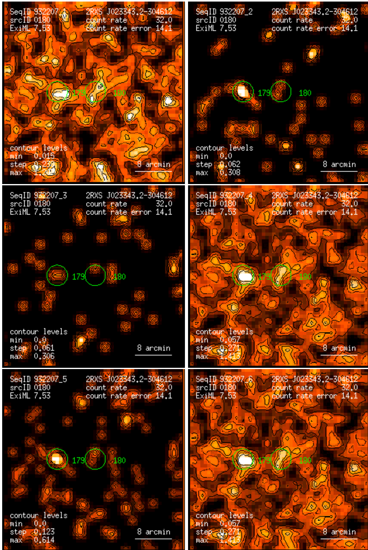
Figure 180: RASS 932207: detection 0180: band rate images, Gaussian filter: (1) PSPC channels 11 – 41, (2) 52 – 90, (3) 91 – 201, (4) 11 – 235, (5) 52 – 201, (6) 11 – 201. Broad band rates in counts/ks. Band rate contour levels in counts/ks/arcmin 2 .
