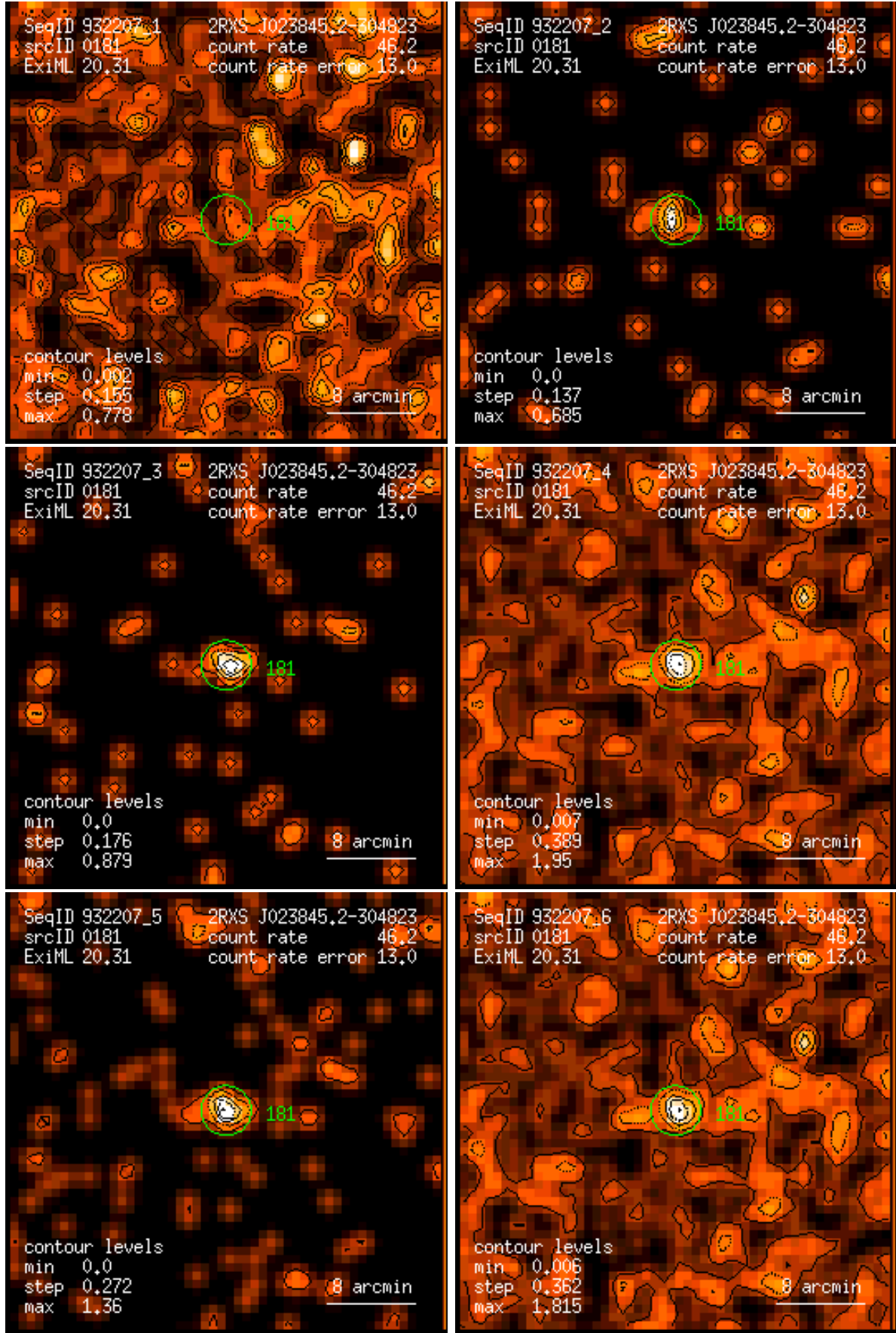
Figure 181: RASS 932207: detection 0181: band rate images, Gaussian filter: (1) PSPC channels 11 – 41, (2) 52 – 90, (3) 91 – 201, (4) 11 – 235, (5) 52 – 201, (6) 11 – 201. Broad band rates in counts/ks. Band rate contour levels in counts/ks/arcmin 2 .
